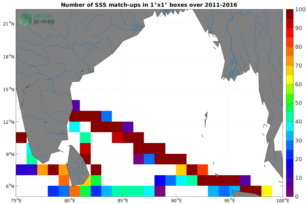
Figure 4: Number of SSS match-ups between TSG (LEGOS-DM) SSS and the SMOS SSS L3 v2 - 9-Days (BEC) SSS product for the Ganga and Brahmaputra river plumes Pi-MEP region over 1°×1° boxes and for the full satellite product period.
