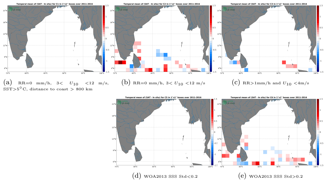
Figure 12: Temporal mean gridded over spatial boxes of size 1°x1° of \Delta SSS (SMOS SSS L3 v2 - 9-Days (BEC) - TSG (LEGOS-DM)) for 5 different subdatasets corresponding to:RR=0 mm/h, 3 < U_{10} < 12 m/s, SST>5°C, distance to coast > 800 km (a), RR=0 mm/h, 3 < U_{10} < 12 m/s (b), RR>1mm/h and U_{10} < 4 m/s (c), WOA2013 SSS Std<0.2 (d), WOA2013 SSS Std>0.2 (e).
