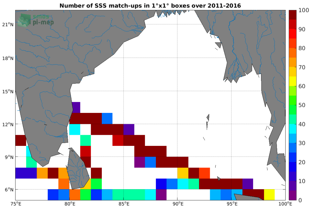
Figure 4: Number of SSS match-ups between TSG (LEGOS-DM) SSS and the SMOS SSS L3 v2 - 9-Days (BEC) SSS product for the Ganga and Brahmaputra river plumes Pi-MEP region over 1°x1° boxes and for the full satellite product period.
