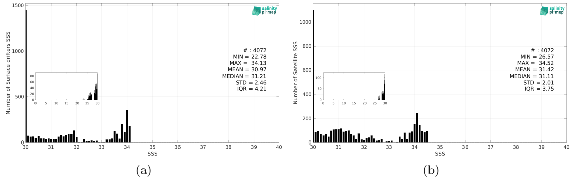
Figure 3: Histograms of SSS from Surface drifters (a) and SMOS SSS L3 v2 - 9-Days (BEC) (b) considering all match-up pairs per bins of 0.1 over the Ganga and Brahmaputra river plumes Pi-MEP region and for the full satellite product period.
