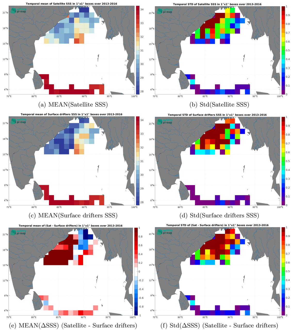
Figure 6: Temporal mean (left) and Std (right) of SSS from SMOS SSS L3 v2 - 9-Days (BEC) (top), Surface drifters (middle), and of \Delta SSS (Satellite - Surface drifters). Only match-up pairs are used to generate these maps.
