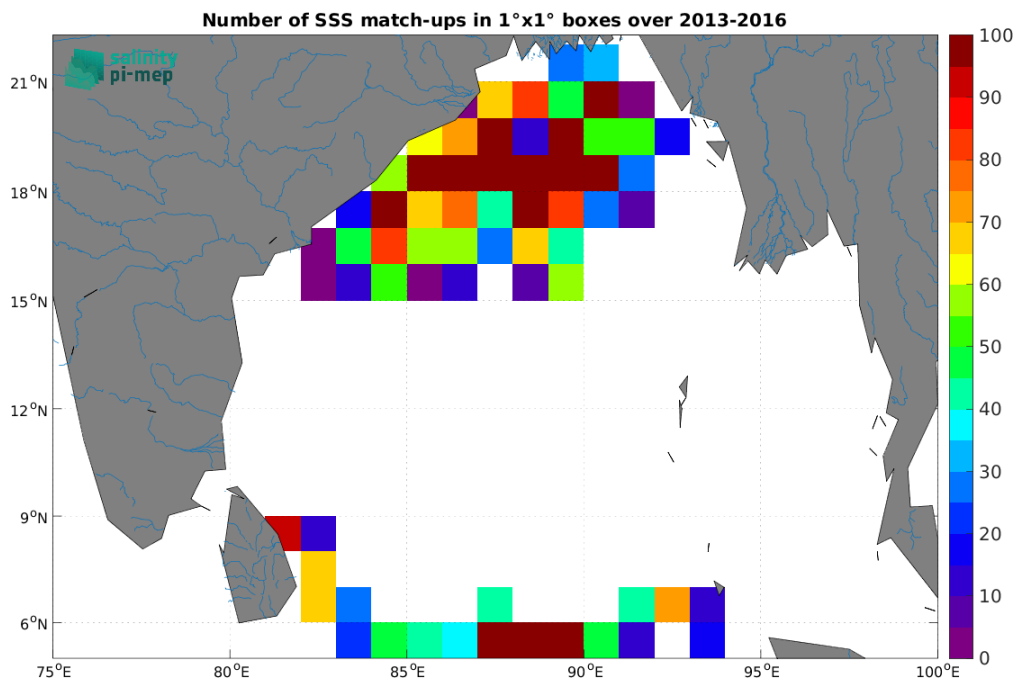
Figure 4: Number of SSS match-ups between Surface drifters SSS and the SMOS SSS L3 v2 - 9-Days (BEC) SSS product for the Ganga and Brahmaputra river plumes Pi-MEP region over 1^\circ \times 1^\circ boxes and for the full satellite product period.
