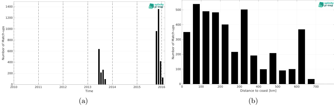
Figure 2: Number of match-ups between Surface drifters and SMOS SSS L3 v2 - 9-Days (BEC) SSS as a function of time (a) and as function of the distance to coast (b) over the Ganga and Brahmaputra river plumes Pi-MEP region and for the full satellite product period.
