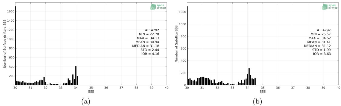
Figure 2: Histograms of SSS from Surface drifters (a) and SMOS L3 v2 - 9-Days (BEC) (b) considering all match-up pairs per bins of 0.1 over the Ganga and Brahmaputra river plumes Pi-MEP region and for the full satellite product period.
