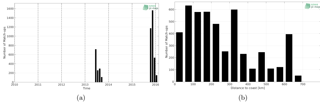
Figure 1: Number of match-ups between Surface drifters and SMOS L3 v2 - 9-Days (BEC) SSS as a function of time (a) and as function of the distance to coast (b) over the Ganga and Brahmaputra river plumes Pi-MEP region and for the full satellite product period.
