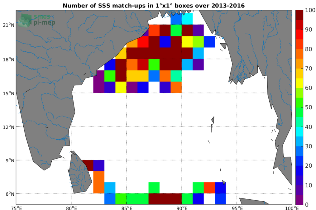
Figure 3: Number of SSS match-ups between Surface drifters SSS and the SMOS L3 v2 - 9-Days (BEC) SSS product for the Ganga and Brahmaputra river plumes Pi-MEP region over 1°x1° boxes and for the full satellite product period.
