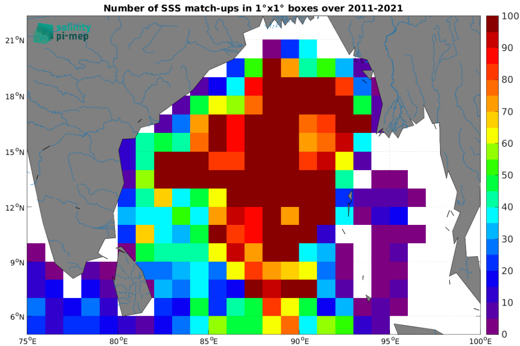
Figure 5: Number of SSS match-ups between Argo SSS and the SMOS SSS L3 v2 - 9-Days (BEC) SSS product for the Ganga and Brahmaputra river plumes Pi-MEP region over 1^{\circ} \times 1^{\circ} boxes and for the full satellite product period.
