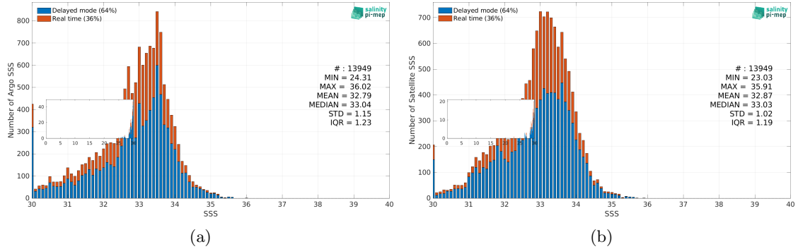
Figure 3: Histograms of SSS from Argo (a) and SMOS SSS L3 v2 - 9-Days (BEC) (b) considering all match-up pairs per bins of 0.1 over the Ganga and Brahmaputra river plumes Pi-MEP region and for the full satellite product period.
