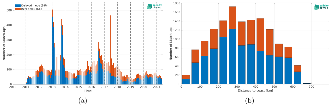
Figure 2: Number of match-ups between Argo and SMOS SSS L3 v2 - 9-Days (BEC) SSS as a function of time (a) and as function of the distance to coast (b) over the Ganga and Brahmaputra river plumes Pi-MEP region and for the full satellite product period.
