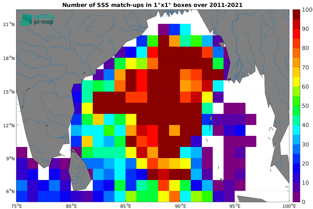
Figure 5: Number of SSS match-ups between Argo SSS and the SMOS SSS L3 v2 - 9-Days (BEC) SSS product for the Ganga and Brahmaputra river plumes Pi-MEP region over 1^\circ \times 1^\circ boxes and for the full satellite product period.
