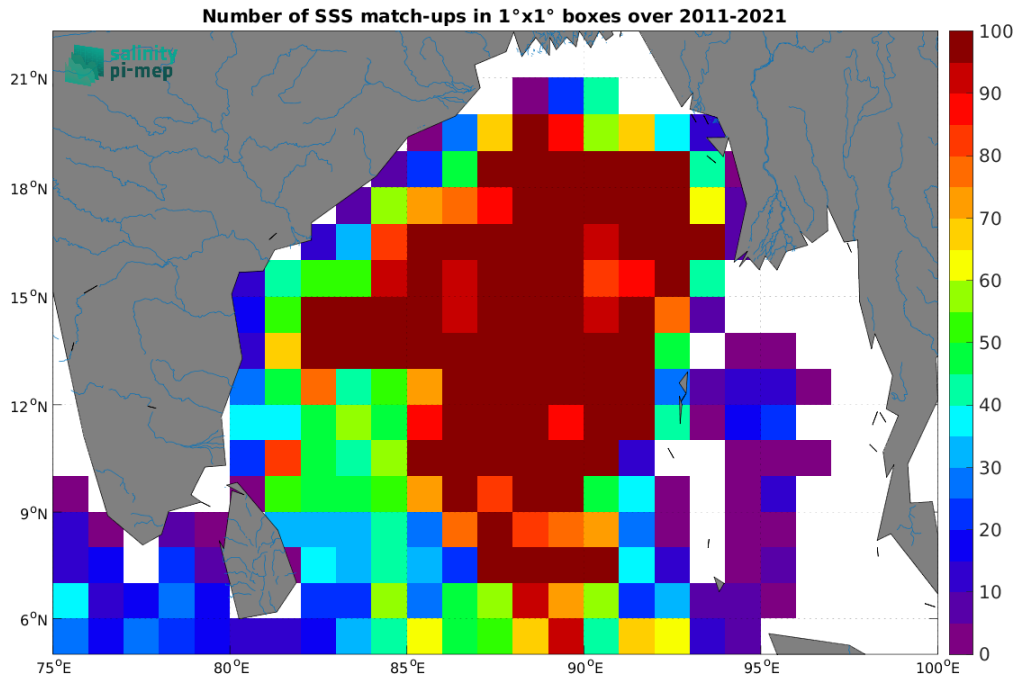
Figure 4: Number of SSS match-ups between Argo SSS and the SMOS SSS L3 v2 - 9-Days (BEC) SSS product for the Ganga and Brahmaputra river plumes Pi-MEP region over 1^\circ \times 1^\circ boxes and for the full satellite product period.
