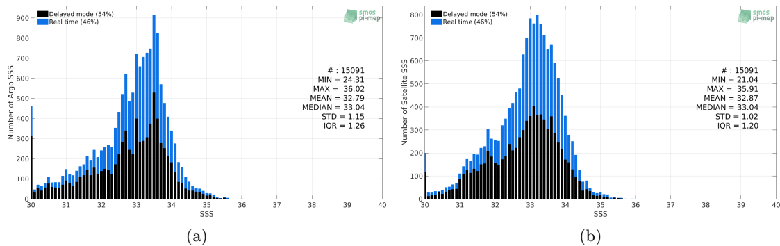
Figure 2: Histograms of SSS from Argo (a) and SMOS L3 v2 - 9-Days (BEC) (b) considering all match-up pairs per bins of 0.1 over the Ganga and Brahmaputra river plumes Pi-MEP region and for the full satellite product period.
