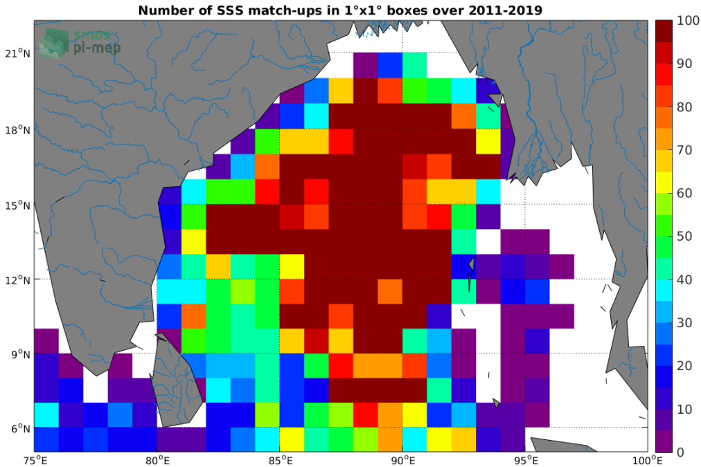
Figure 4: Number of SSS match-ups between Argo SSS and the SMOS L3 v2 - 9-Days (BEC) SSS product for the Ganga and Brahmaputra river plumes Pi-MEP region over 1°x1° boxes and for the full satellite product period.
