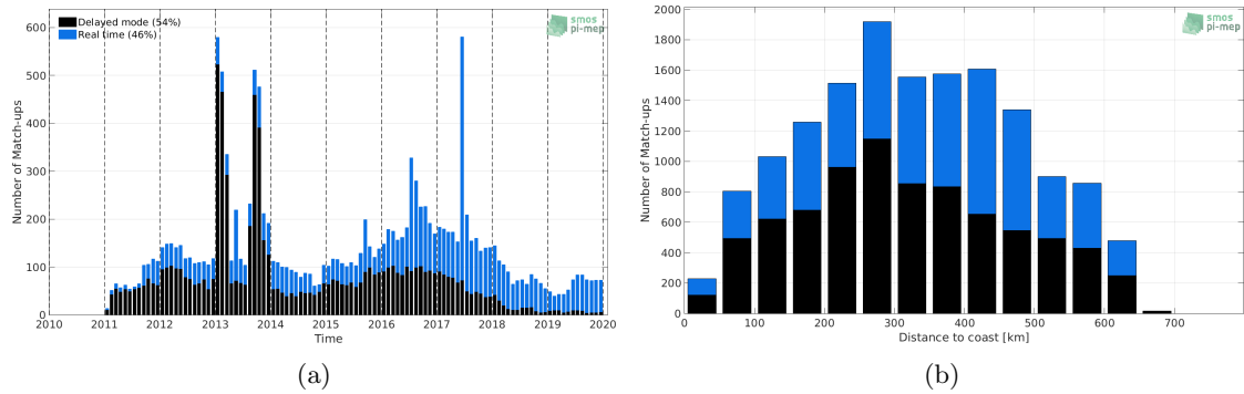
Figure 1: Number of match-ups between Argo and SMOS L3 v2 - 9-Days (BEC) SSS as a function of time (a) and as function of the distance to coast (b) over the Ganga and Brahmaputra river plumes Pi-MEP region and for the full satellite product period.
