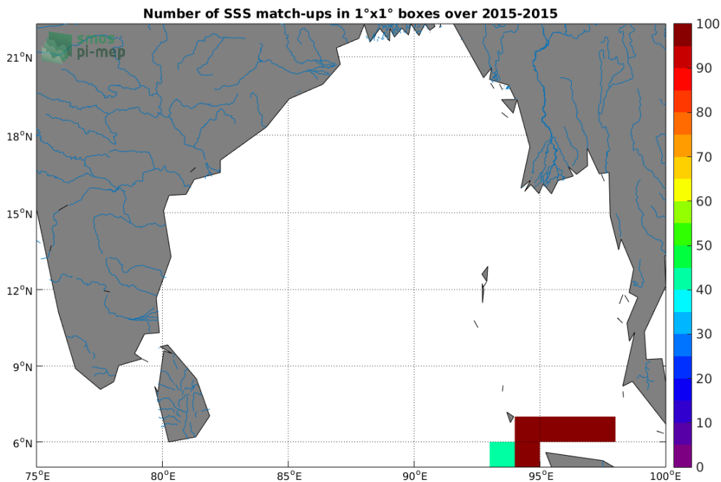
Figure 4: Number of SSS match-ups between TSG-SAMOS SSS and the SMOS-L3-BEC-OA-V1-9DAYS-0.25DEG SSS product for the Ganga and Brahmaputra river plumes Pi-MEP region over 1°x1° boxes and for the full satellite product period.
