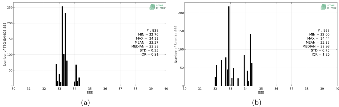
Figure 2: Histograms of SSS from TSG-SAMOS (a) and SMOS-L3-BEC-OA-V1-9DAYS-0.25DEG (b) considering all match-up pairs per bins of 0.1 over the Ganga and Brahmaputra river plumes Pi-MEP region and for the full satellite product period.
