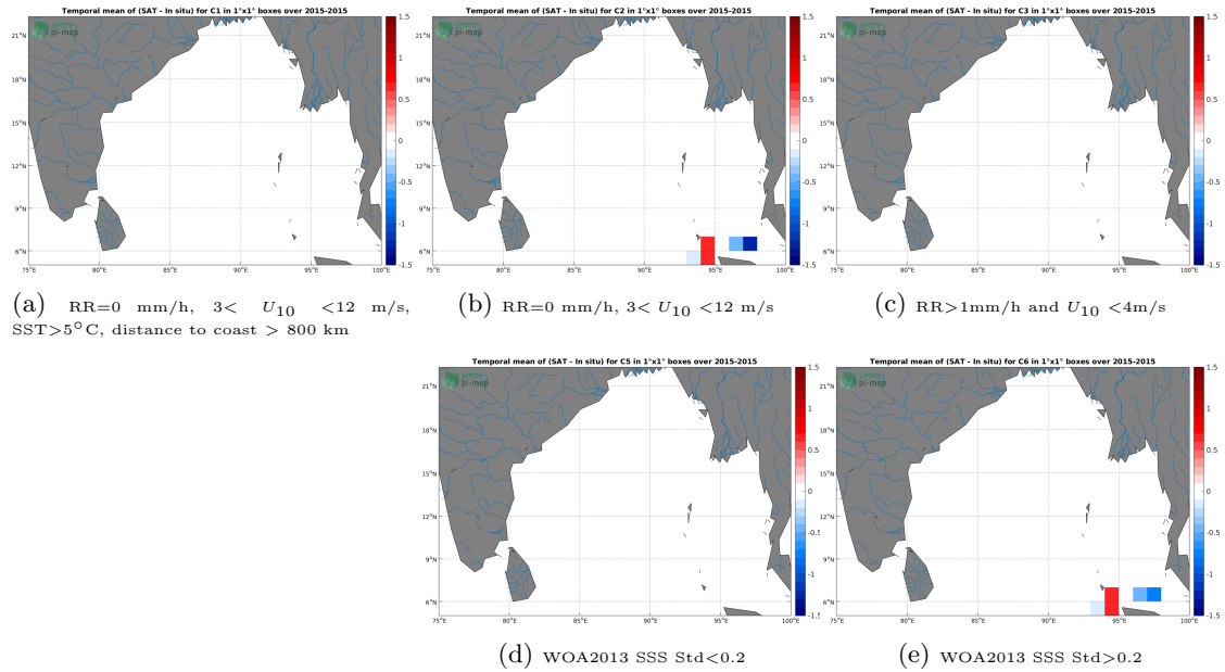
Figure 12: Temporal mean gridded over spatial boxes of size 1^\circ \times 1^\circ of \Delta SSS (SMOS-L3-BEC-OA-V1-9DAYS-0.25DEG - TSG-SAMOS) for 5 different subdatasets corresponding to:RR=0 mm/h, 3 < U_{10} < 12 m/s, SST >5^\circ C, distance to coast > 800 km (a), RR=0 mm/h, 3 < U_{10} < 12 m/s (b), RR >1 mm/h and U_{10} < 4 m/s (c), WOA2013 SSS Std <0.2 (d), WOA2013 SSS Std >0.2 (e).
