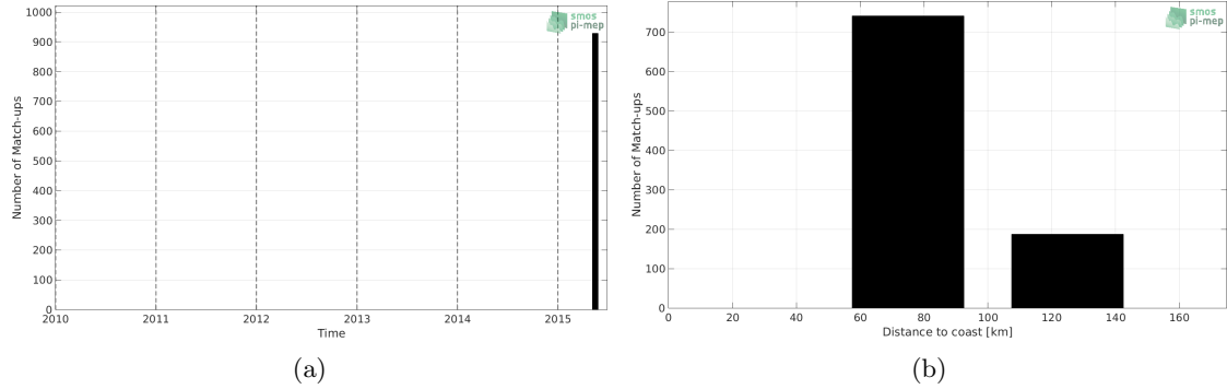
Figure 1: Number of match-ups between TSG-SAMOS and SMOS-L3-BEC-OA-V1-9DAYS-0.25DEG SSS as a function of time (a) and as function of the distance to coast (b) over the Ganga and Brahmaputra river plumes Pi-MEP region and for the full satellite product period.
