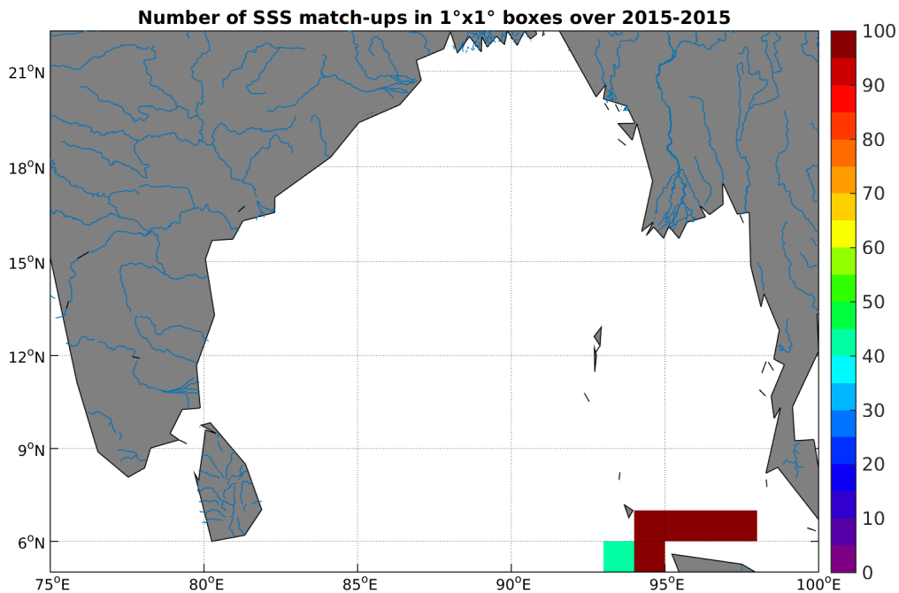
Figure 4: Number of SSS match-ups between TSG-SAMOS SSS and the SMOS-L3-BEC-OA-V1-9DAYS-0.25DEG SSS product for the Ganga and Brahmaputra river plumes Pi-MEP region over 1^{\circ} \times 1^{\circ} boxes and for the full satellite product period.
