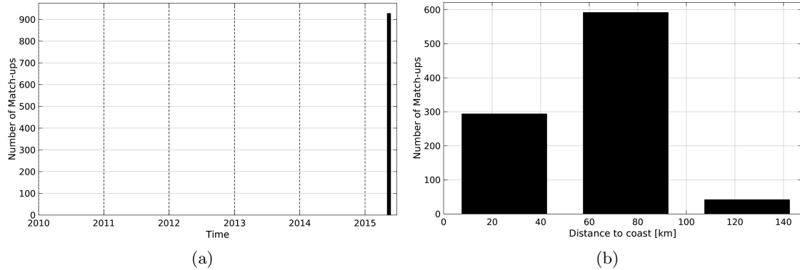
Figure 1: Number of match-ups between TSG-SAMOS and SMOS-L3-BEC-OA-V1-9DAYS-0.25DEG SSS as a function of time (a) and as function of the distance to coast (b) over the Ganga and Brahmaputra river plumes Pi-MEP region and for the full satellite product period.
