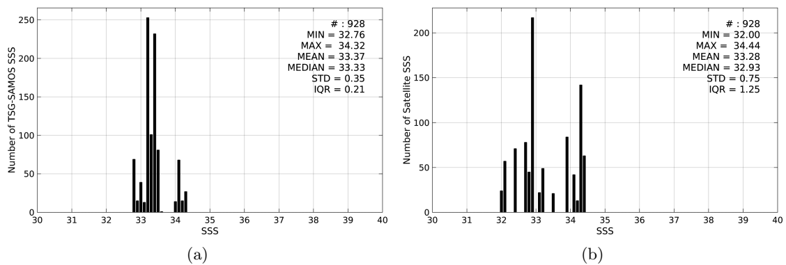
Figure 2: Histograms of SSS from TSG-SAMOS (a) and SMOS-L3-BEC-OA-V1-9DAYS-0.25DEG (b) considering all match-up pairs per bins of 0.1 over the Ganga and Brahmaputra river plumes Pi-MEP region and for the full satellite product period.
