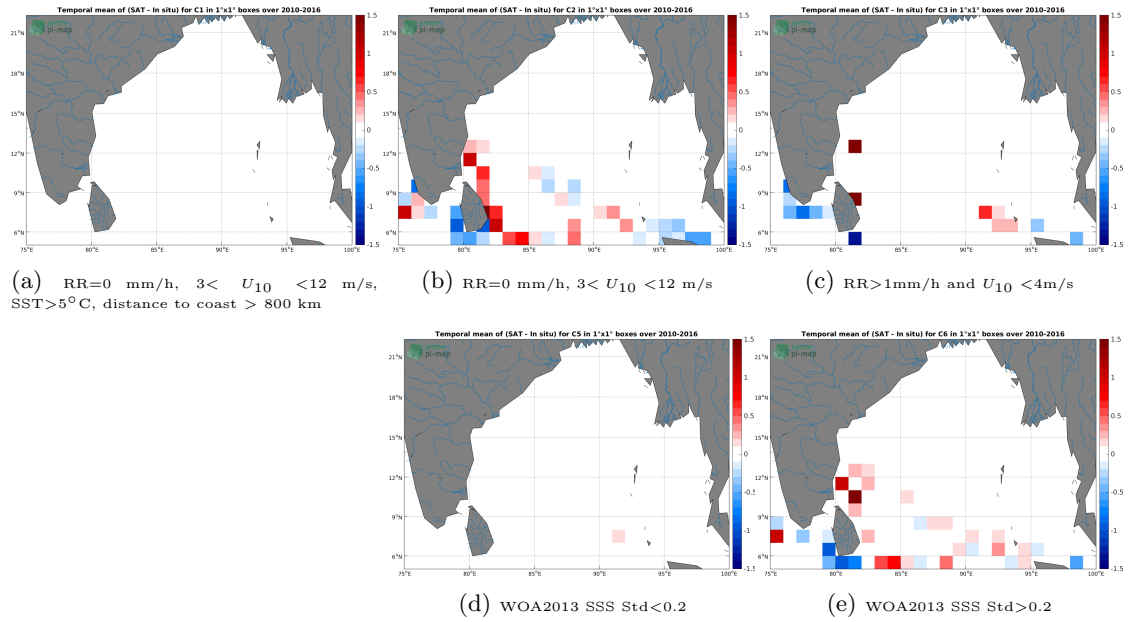
Figure 12: Temporal mean gridded over spatial boxes of size 1^\circ \times 1^\circ of \Delta SSS (SMOS-L3-BEC-OA-V1-9DAYS-0.25DEG - TSG-LEGOS-DM) for 5 different subdatasets corresponding to:RR=0 mm/h, 3 < U_{10} < 12 m/s, SST > 5^\circ\text{C} , distance to coast > 800 km (a), RR=0 mm/h, 3 < U_{10} < 12 m/s (b), RR > 1 mm/h and U_{10} < 4 m/s (c), WOA2013 SSS Std < 0.2 (d), WOA2013 SSS Std > 0.2 (e).
