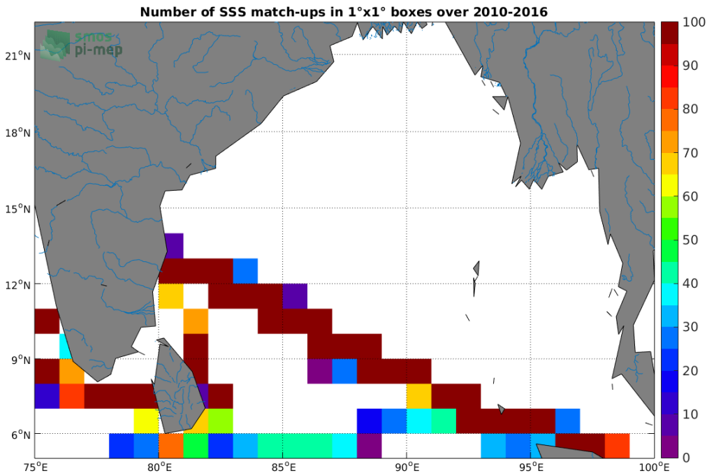
Figure 4: Number of SSS match-ups between TSG-LEGOS-DM SSS and the SMOS-L3-BEC-OA-V1-9DAYS-0.25DEG SSS product for the Ganga and Brahmaputra river plumes Pi-MEP region over 1^\circ \times 1^\circ boxes and for the full satellite product period.
