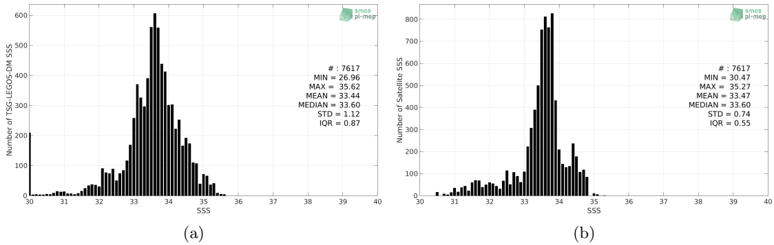
Figure 2: Histograms of SSS from TSG-LEGOS-DM (a) and SMOS-L3-BEC-OA-V1-9DAYS-0.25DEG (b) considering all match-up pairs per bins of 0.1 over the Ganga and Brahmaputra river plumes Pi-MEP region and for the full satellite product period.
