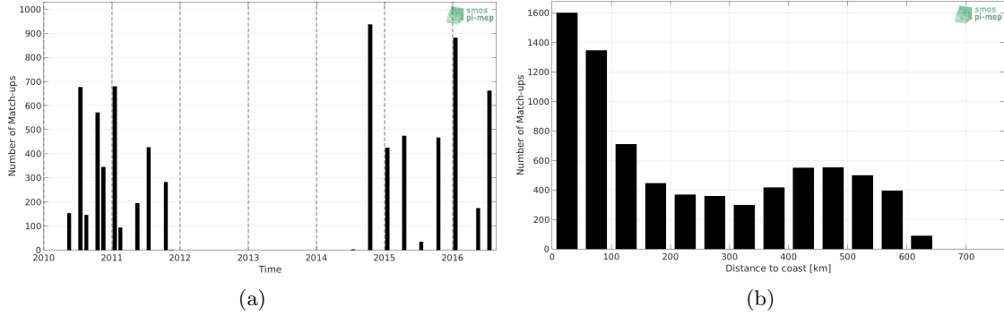
Figure 1: Number of match-ups between TSG-LEGOS-DM and SMOS-L3-BEC-OA-V1-9DAYS-0.25DEG SSS as a function of time (a) and as function of the distance to coast (b) over the Ganga and Brahmaputra river plumes Pi-MEP region and for the full satellite product period.
