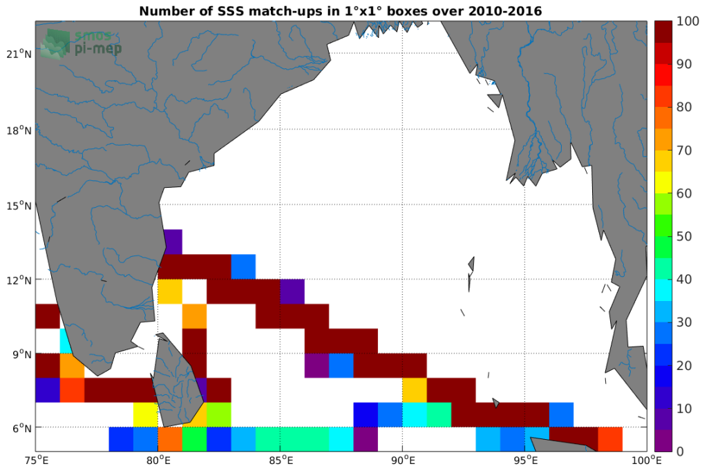
Figure 4: Number of SSS match-ups between TSG-LEGOS-DM SSS and the SMOS-L3-BEC-OA-V1-9DAYS-0.25DEG SSS product for the Ganga and Brahmaputra river plumes Pi-MEP region over 1°x1° boxes and for the full satellite product period.
