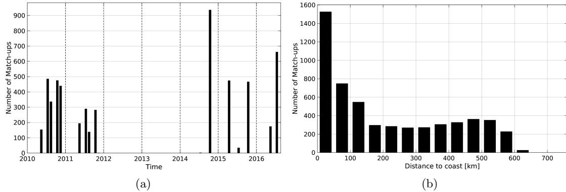
Figure 1: Number of match-ups between TSG-LEGOS-DM and SMOS-L3-BEC-OA-V1-9DAYS-0.25DEG SSS as a function of time (a) and as function of the distance to coast (b) over the Ganga and Brahmaputra river plumes Pi-MEP region and for the full satellite product period.
