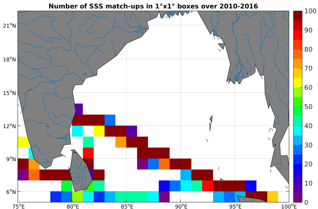
Figure 4: Number of SSS match-ups between TSG-LEGOS-DM SSS and the SMOS-L3-BEC-OA-V1-9DAYS-0.25DEG SSS product for the Ganga and Brahmaputra river plumes Pi-MEP region over 1^{\circ} \times 1^{\circ} boxes and for the full satellite product period.
