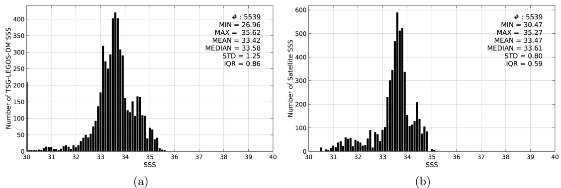
Figure 2: Histograms of SSS from TSG-LEGOS-DM (a) and SMOS-L3-BEC-OA-V1-9DAYS-0.25DEG (b) considering all match-up pairs per bins of 0.1 over the Ganga and Brahmaputra river plumes Pi-MEP region and for the full satellite product period.
