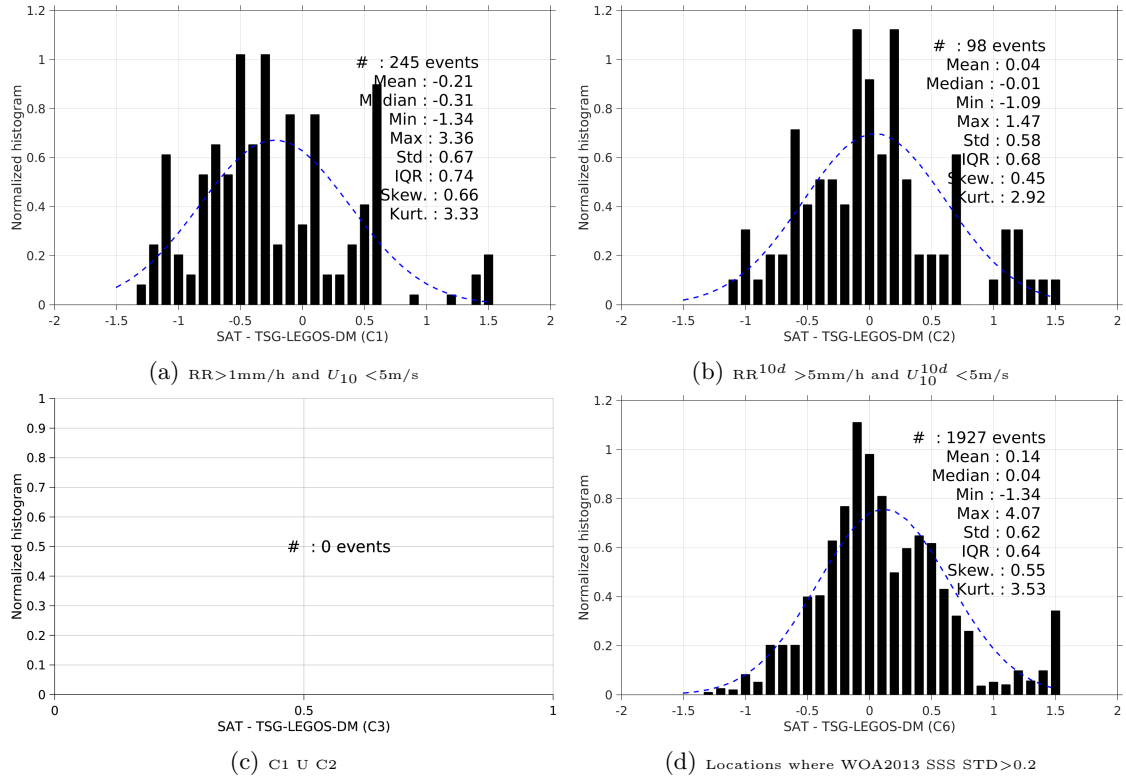
Figure 13: Normalized histogram of \Delta\text{SSS} (SMOS-L3-BEC-OA-V1-9DAYS-0.25DEG - TSG-LEGOS-DM) for 6 different subdatasets corresponding to: RR>1mm/h and U_{10} < 5\text{m/s} (a), RR^{10d} > 5\text{mm/h} and U_{10}^{10d} < 5\text{m/s} (b), C1 U C2 (c), Locations where WOA2013 SSS STD>0.2 (d).
