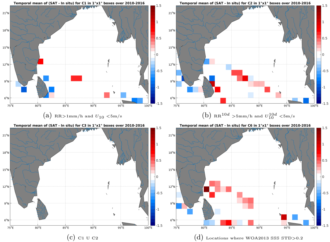
Figure 12: Temporal mean gridded over spatial boxes of size 1°x1° of \Delta SSS (SMOS-L3-BEC-OA-V1-9DAYS-0.25DEG - TSG-LEGOS-DM) for 4 different subdatasets corresponding to: RR > 1mm/h and U_{10} < 5\text{m/s} (a), RR^{10d} > 5\text{mm/h} and U_{10}^{10d} < 5\text{m/s} (b), C1 U C2 (c), Locations where WOA2013 SSS STD > 0.2 (d).
