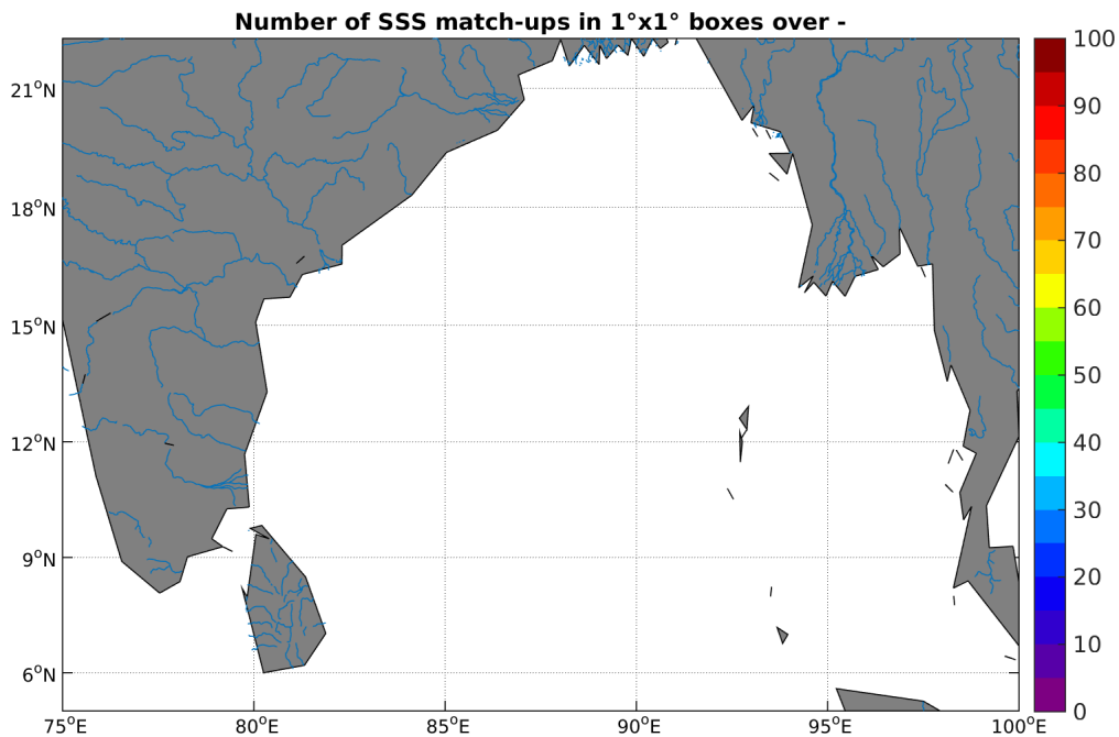
Figure 4: Number of SSS match-ups between TSG-GOSUD-Research-vessel SSS and the SMOS-L3-BEC-OA-V1-9DAYS-0.25DEG SSS product for the Ganga and Brahmaputra river plumes Pi-MEP region over 1°x1° boxes and for the full satellite product period.
