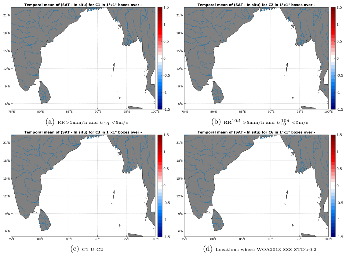
Figure 12: Temporal mean gridded over spatial boxes of size 1^\circ \times 1^\circ of \Delta SSS (SMOS-L3-BEC-OA-V1-9DAYS-0.25DEG - TSG-GOSUD-Research-vessel) for 4 different subdatasets corresponding to:RR > 1 mm/h and U_{10} < 5 m/s (a), RR^{10d} > 5 mm/h and U_{10}^{10d} < 5 m/s (b), C1 U C2 (c),Locations where WOA2013 SSS STD > 0.2 (d).
