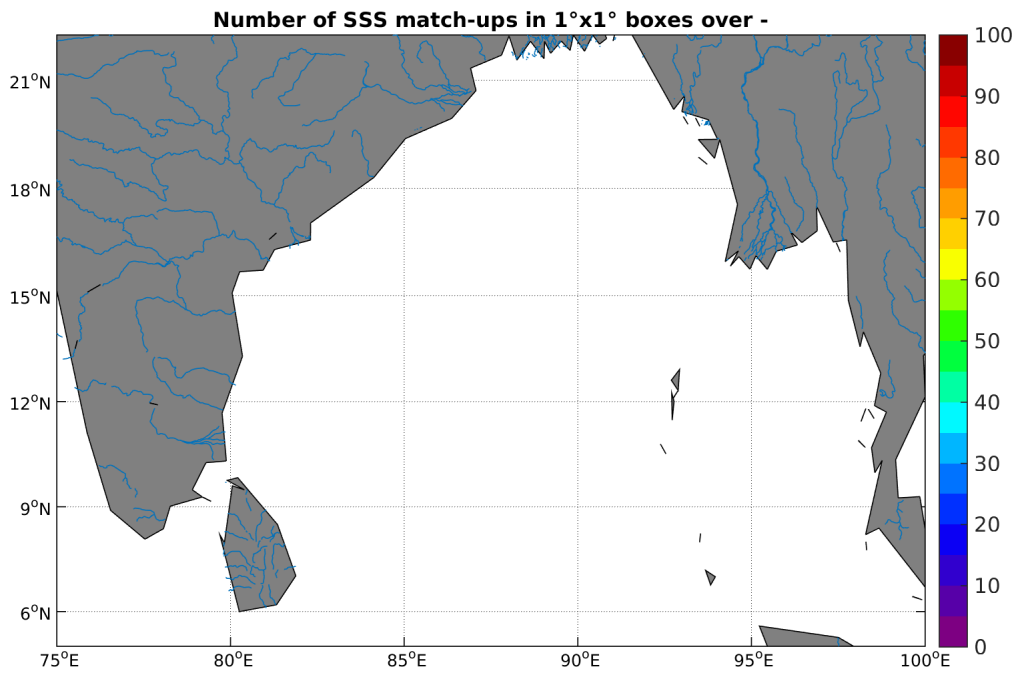
Figure 4: Number of SSS match-ups between Sea mammals SSS and the SMOS-L3-BEC-OA-V1-9DAYS-0.25DEG SSS product for the Ganga and Brahmaputra river plumes Pi-MEP region over 1^\circ \times 1^\circ boxes and for the full satellite product period.
