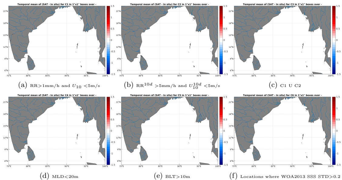
Figure 12: Temporal mean gridded over spatial boxes of size 1^\circ \times 1^\circ of \Delta SSS (SMOS-L3-BEC-OA-V1-9DAYS-0.25DEG - Sea mammals) for 6 different subdatasets corresponding to:RR > 1 mm/h and U_{10} < 5 m/s (a), RR 10d > 5 mm/h and U_{10}^{10d} < 5 m/s (b), C1 U C2 (c),MLD < 20 m (d),BLT > 10 m (e),Locations where WOA2013 SSS STD > 0.2 (f).
