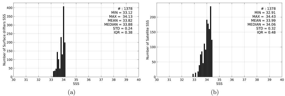
Figure 2: Histograms of SSS from Surface drifters (a) and SMOS-L3-BEC-OA-V1-9DAYS-0.25DEG (b) considering all match-up pairs per bins of 0.1 over the Ganga and Brahmaputra river plumes Pi-MEP region and for the full satellite product period.
