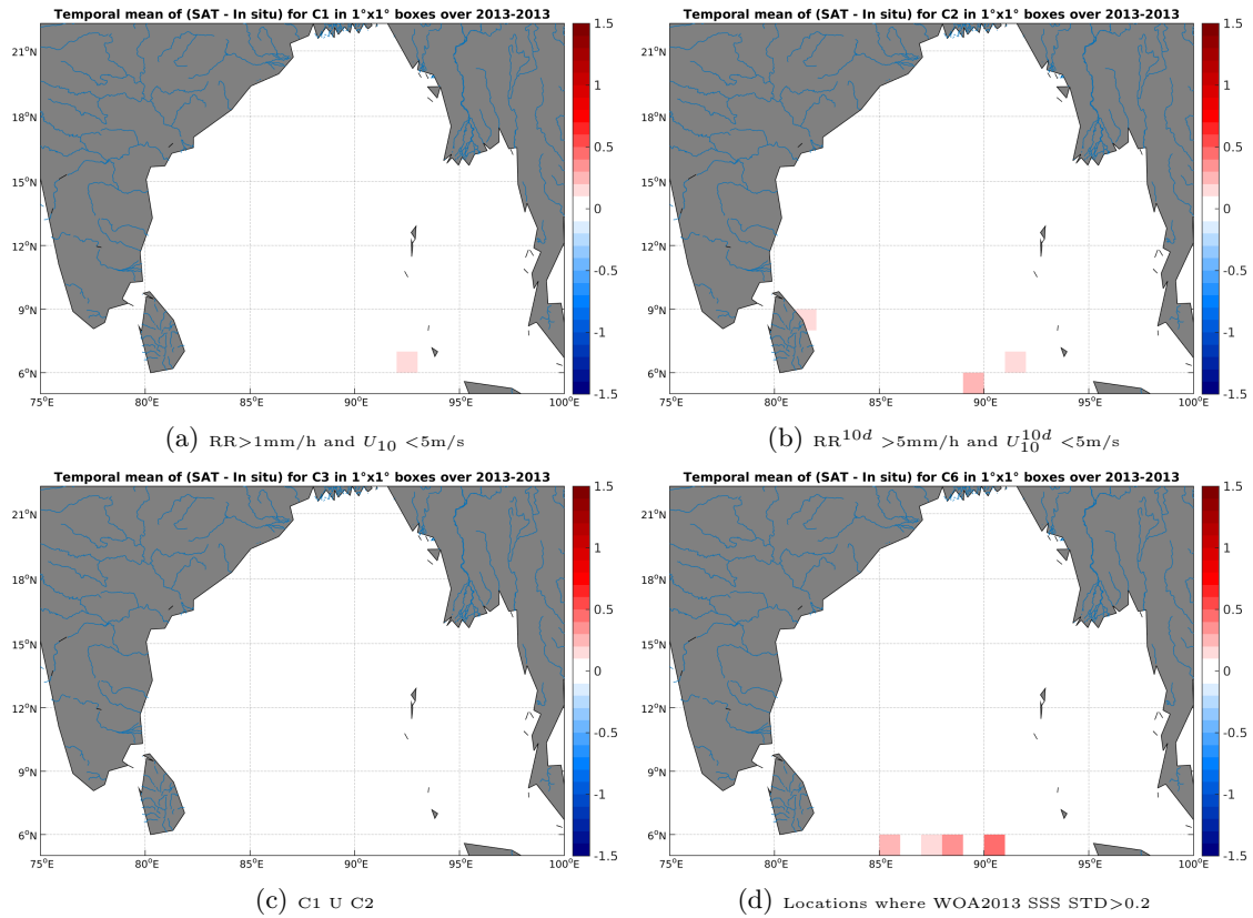
Figure 11: Temporal mean gridded over spatial boxes of size 1°x1° of \Delta SSS (SMOS-L3-BEC-OA-V1-9DAYS-0.25DEG - Surface drifters) for 4 different subdatasets corresponding to:RR>1mm/h and U_{10} < 5\text{m/s} (a), RR^{10d} > 5\text{mm/h} and U_{10}^{10d} < 5\text{m/s} (b), C1 U C2 (c),Locations where WOA2013 SSS STD>0.2 (d).
