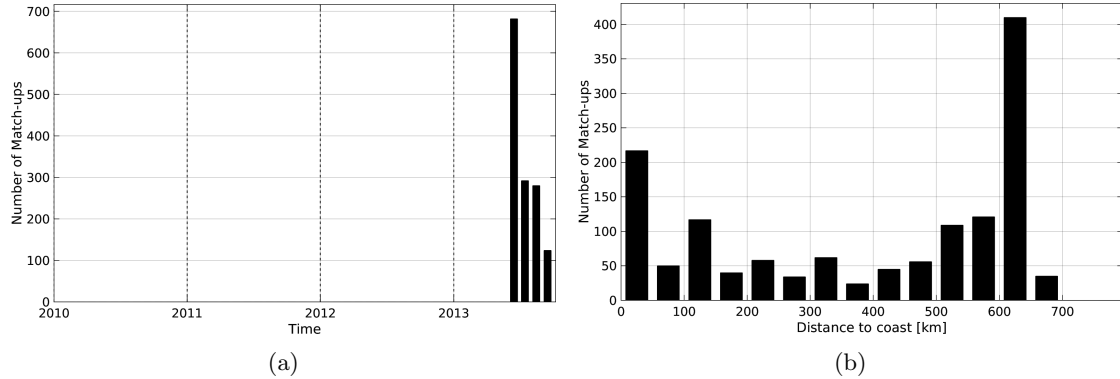
Figure 1: Number of match-ups between Surface drifters and SMOS-L3-BEC-OA-V1-9DAYS-0.25DEG SSS as a function of time (a) and as function of the distance to coast (b) over the Ganga and Brahmaputra river plumes Pi-MEP region and for the full satellite product period.
