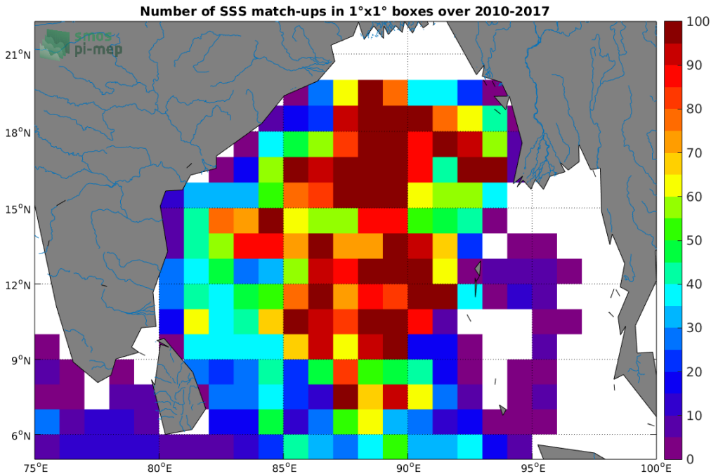
Figure 4: Number of SSS match-ups between Argo SSS and the SMOS-L3-BEC-OA-V1-9DAYS-0.25DEG SSS product for the Ganga and Brahmaputra river plumes Pi-MEP region over 1°x1° boxes and for the full satellite product period.
