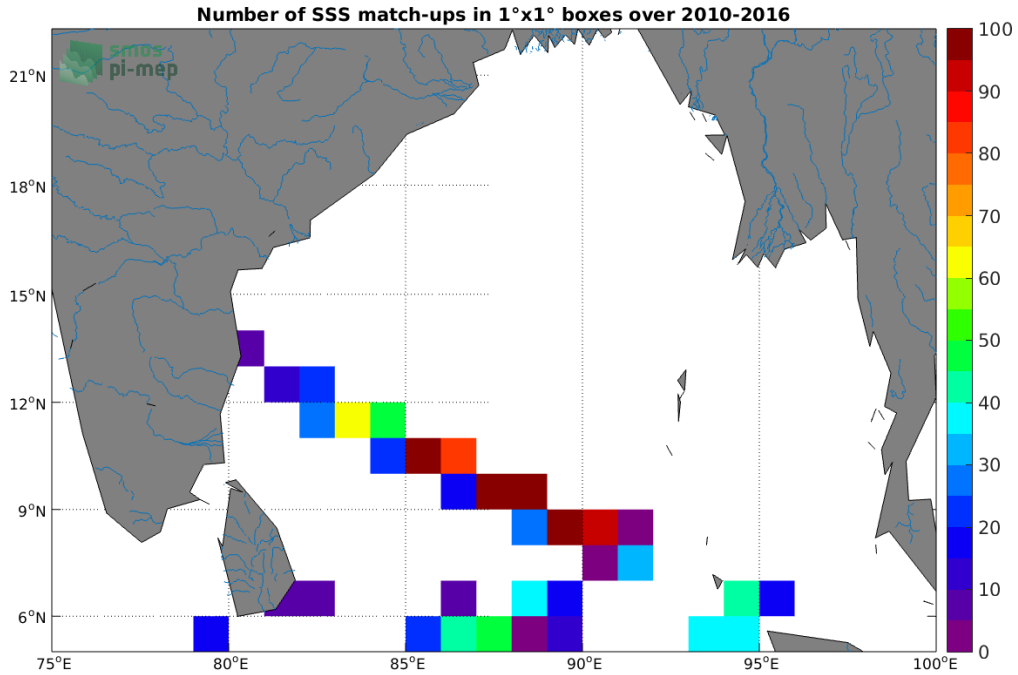
Figure 4: Number of SSS match-ups between TSG (LEGOS-DM) SSS and the SMOS SSS L2 v700 (ESA) SSS product for the Ganga and Brahmaputra river plumes Pi-MEP region over 1^\circ \times 1^\circ boxes and for the full satellite product period.
