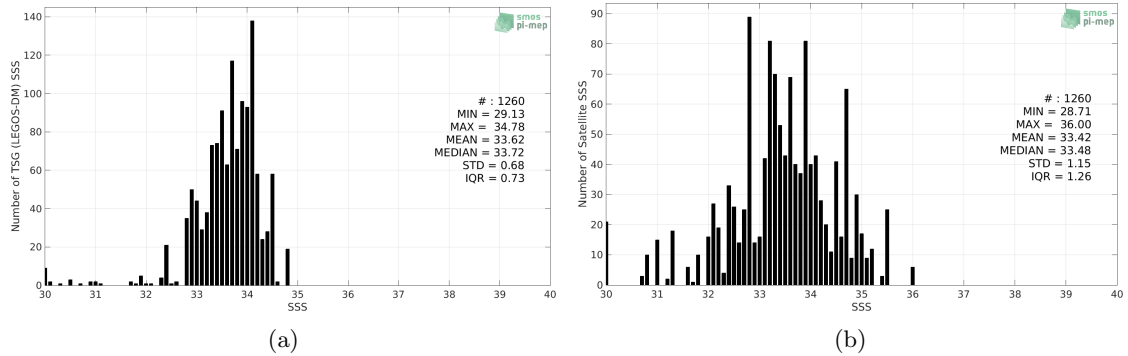
Figure 2: Histograms of SSS from TSG (LEGOS-DM) (a) and SMOS SSS L2 v700 (ESA) (b) considering all match-up pairs per bins of 0.1 over the Ganga and Brahmaputra river plumes Pi-MEP region and for the full satellite product period.
