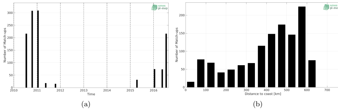
Figure 1: Number of match-ups between TSG (LEGOS-DM) and SMOS SSS L2 v700 (ESA) SSS as a function of time (a) and as function of the distance to coast (b) over the Ganga and Brahmaputra river plumes Pi-MEP region and for the full satellite product period.
