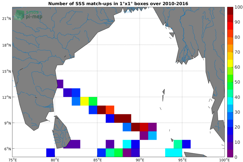
Figure 4: Number of SSS match-ups between TSG (LEGOS-DM) SSS and the SMOS SSS L2 v700 (ESA) SSS product for the Ganga and Brahmaputra river plumes Pi-MEP region over 1°x1° boxes and for the full satellite product period.
