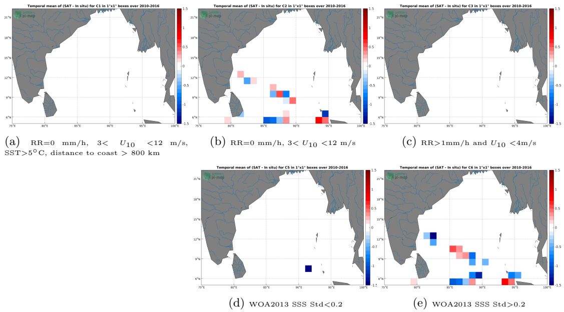
Figure 12: Temporal mean gridded over spatial boxes of size 1°x1° of \Delta SSS (SMOS SSS L2 v700 (ESA) - TSG (LEGOS-DM)) for 5 different subdatasets corresponding to:RR=0 mm/h, 3 < U_{10} < 12 m/s, SST>5°C, distance to coast > 800 km (a), RR=0 mm/h, 3 < U_{10} < 12 m/s (b), RR>1mm/h and U_{10} < 4 m/s (c), WOA2013 SSS Std<0.2 (d), WOA2013 SSS Std>0.2 (e).
