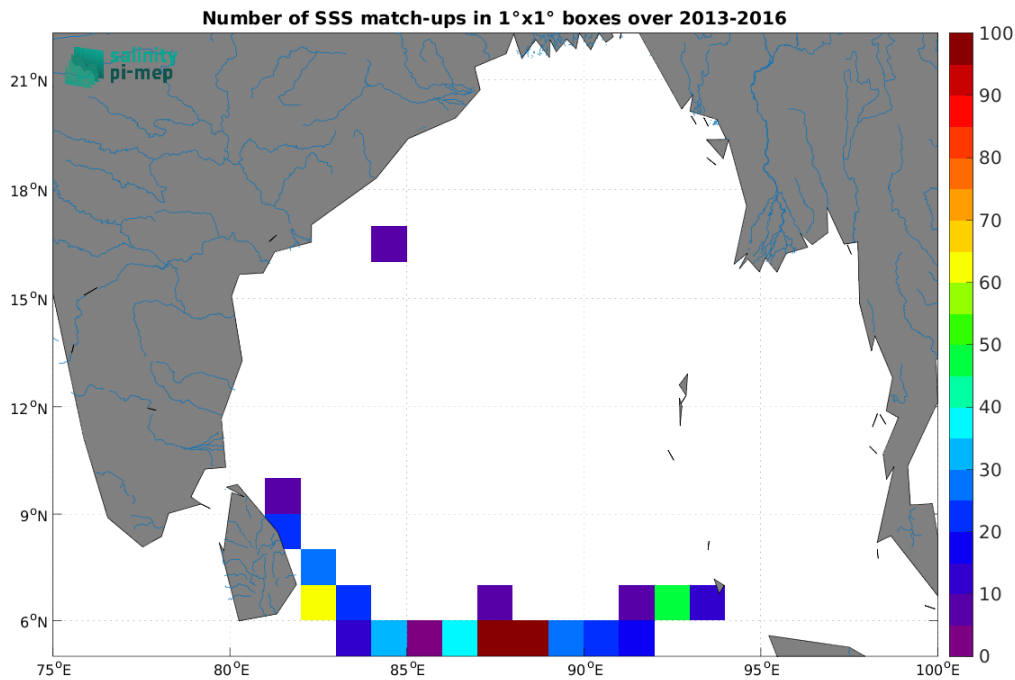
Figure 3: Number of SSS match-ups between Surface drifters SSS and the SMOS SSS L2 v700 (ESA) SSS product for the Ganga and Brahmaputra river plumes Pi-MEP region over 1^\circ \times 1^\circ boxes and for the full satellite product period.
