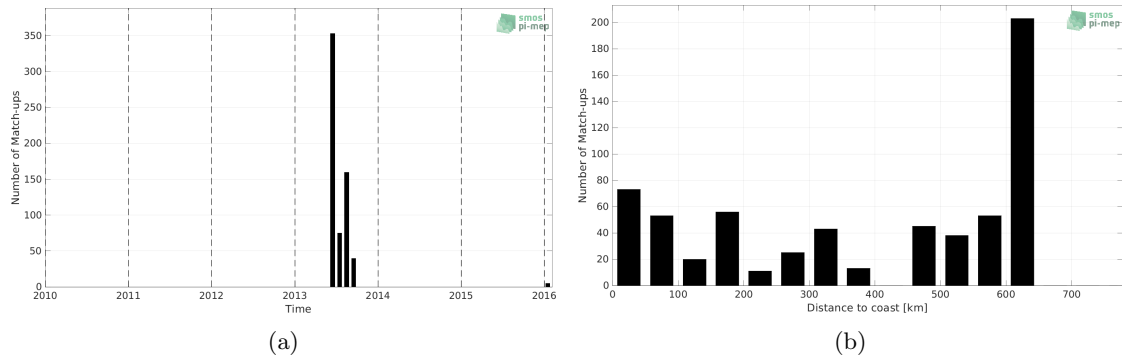
Figure 1: Number of match-ups between Surface drifters and SMOS SSS L2 v700 (ESA) SSS as a function of time (a) and as function of the distance to coast (b) over the Ganga and Brahmaputra river plumes Pi-MEP region and for the full satellite product period.
