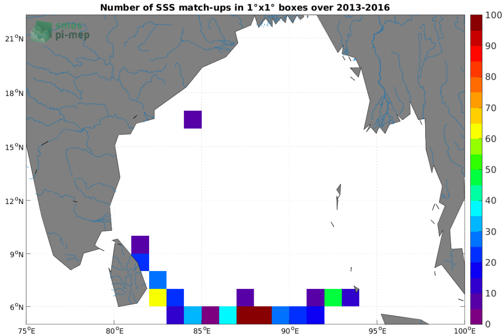
Figure 3: Number of SSS match-ups between Surface drifters SSS and the SMOS SSS L2 v700 (ESA) SSS product for the Ganga and Brahmaputra river plumes Pi-MEP region over 1°x1° boxes and for the full satellite product period.
