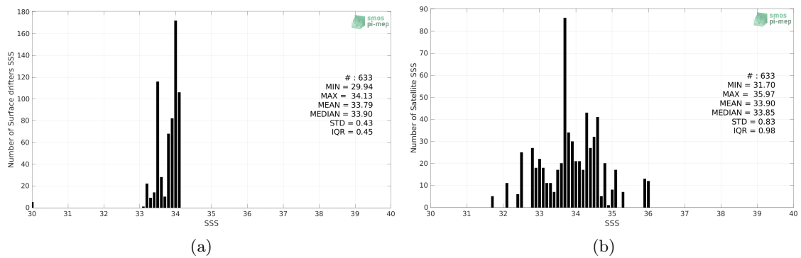
Figure 2: Histograms of SSS from Surface drifters (a) and SMOS SSS L2 v700 (ESA) (b) considering all match-up pairs per bins of 0.1 over the Ganga and Brahmaputra river plumes Pi-MEP region and for the full satellite product period.
