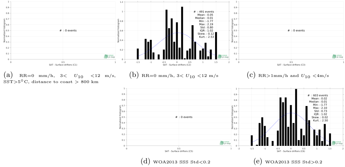
Figure 12: Normalized histogram of \Delta\text{SSS} (SMOS SSS L2 v700 (ESA) - Surface drifters) for 5 different subdatasets corresponding to: RR=0 mm/h, 3 < U_{10} < 12 m/s, SST > 5^\circ\text{C} , distance to coast > 800 km (a), RR=0 mm/h, 3 < U_{10} < 12 m/s (b), RR > 1 mm/h and U_{10} < 4 m/s (c), WOA2013 SSS Std < 0.2 (d), WOA2013 SSS Std > 0.2 (e).
