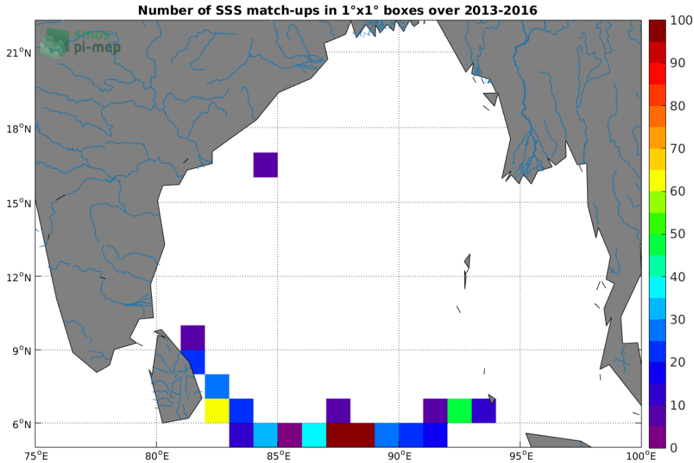
Figure 3: Number of SSS match-ups between Surface drifters SSS and the SMOS SSS L2 v700 (ESA) SSS product for the Ganga and Brahmaputra river plumes Pi-MEP region over 1^{\circ} \times 1^{\circ} boxes and for the full satellite product period.
