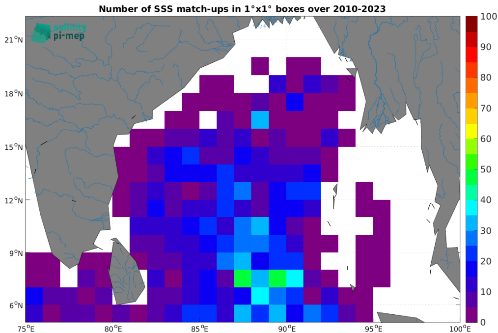
Figure 4: Number of SSS match-ups between Argo SSS and the SMOS SSS L2 v700 (ESA) SSS product for the Ganga and Brahmaputra river plumes Pi-MEP region over 1°×1° boxes and for the full satellite product period.
