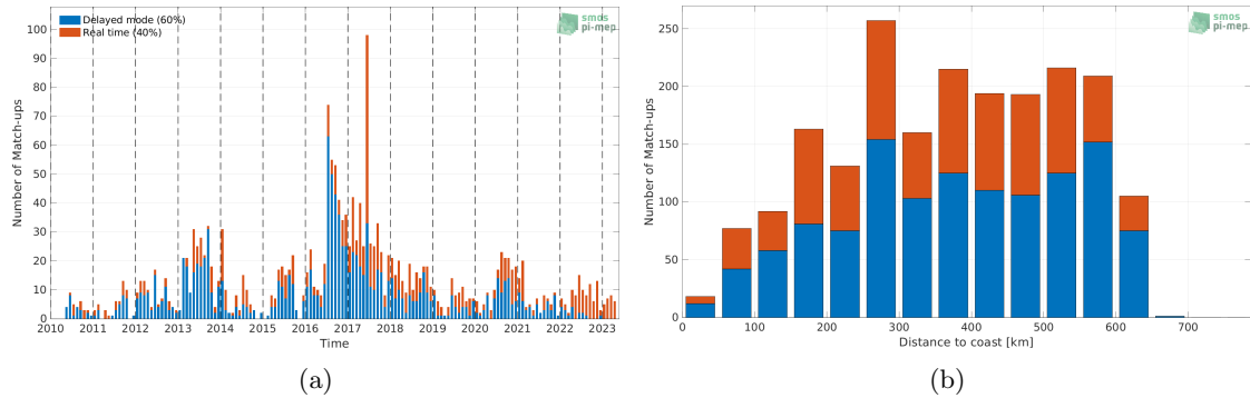
Figure 1: Number of match-ups between Argo and SMOS SSS L2 v700 (ESA) SSS as a function of time (a) and as function of the distance to coast (b) over the Ganga and Brahmaputra river plumes Pi-MEP region and for the full satellite product period.
