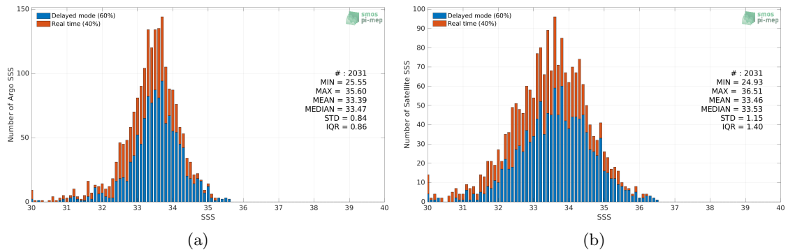
Figure 2: Histograms of SSS from Argo (a) and SMOS SSS L2 v700 (ESA) (b) considering all match-up pairs per bins of 0.1 over the Ganga and Brahmaputra river plumes Pi-MEP region and for the full satellite product period.
