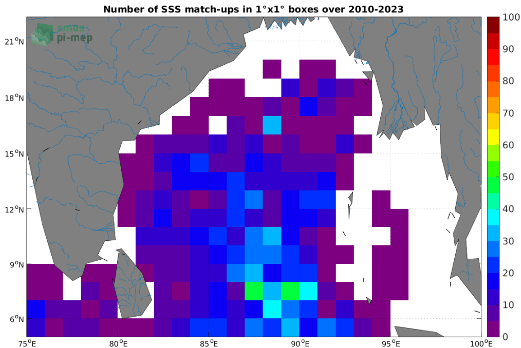
Figure 4: Number of SSS match-ups between Argo SSS and the SMOS SSS L2 v700 (ESA) SSS product for the Ganga and Brahmaputra river plumes Pi-MEP region over 1^\circ \times 1^\circ boxes and for the full satellite product period.
