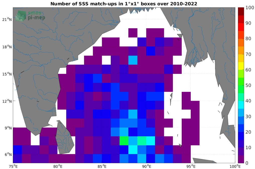
Figure 4: Number of SSS match-ups between Argo SSS and the SMOS SSS L2 v700 (ESA) SSS product for the Ganga and Brahmaputra river plumes Pi-MEP region over 1°x1° boxes and for the full satellite product period.
