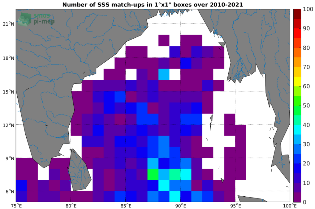
Figure 4: Number of SSS match-ups between Argo SSS and the SMOS SSS L2 v700 (ESA) SSS product for the Ganga and Brahmaputra river plumes Pi-MEP region over 1^{\circ} \times 1^{\circ} boxes and for the full satellite product period.
