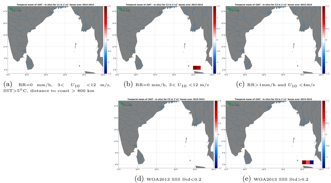
Figure 12: Temporal mean gridded over spatial boxes of size 1°x1° of \Delta SSS (SMOS SSS L2 v662 (ESA) - TSG (SAMOS)) for 5 different subdatasets corresponding to:RR=0 mm/h, 3 < U_{10} < 12 m/s, SST>5°C, distance to coast > 800 km (a), RR=0 mm/h, 3 < U_{10} < 12 m/s (b), RR>1mm/h and U_{10} < 4 m/s (c), WOA2013 SSS Std<0.2 (d), WOA2013 SSS Std>0.2 (e).
