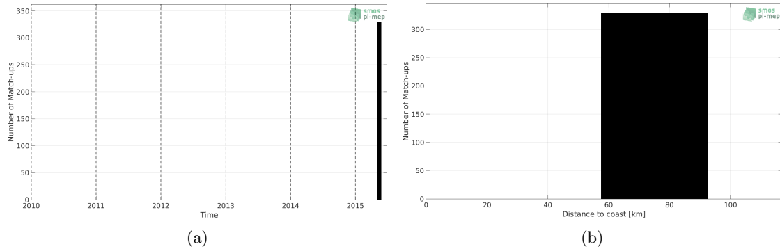
Figure 1: Number of match-ups between TSG (SAMOS) and SMOS SSS L2 v662 (ESA) SSS as a function of time (a) and as function of the distance to coast (b) over the Ganga and Brahmaputra river plumes Pi-MEP region and for the full satellite product period.
