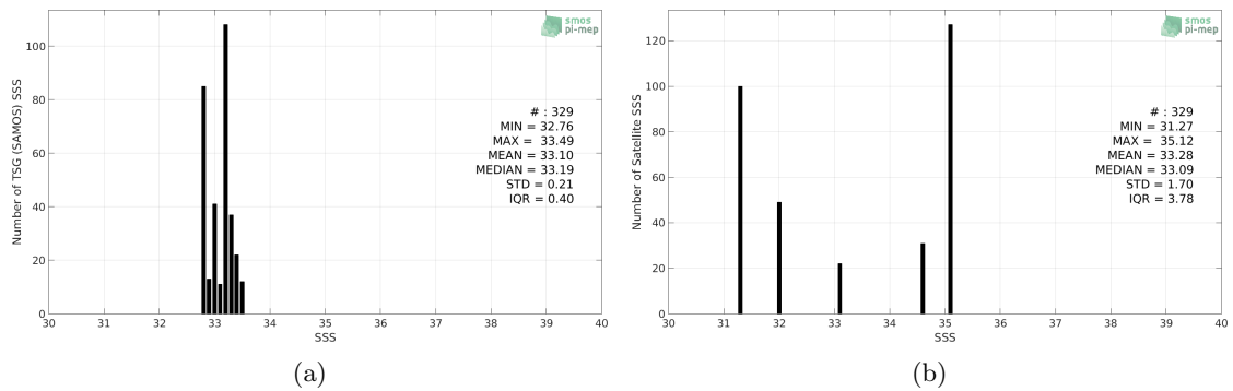
Figure 2: Histograms of SSS from TSG (SAMOS) (a) and SMOS SSS L2 v662 (ESA) (b) considering all match-up pairs per bins of 0.1 over the Ganga and Brahmaputra river plumes Pi-MEP region and for the full satellite product period.
