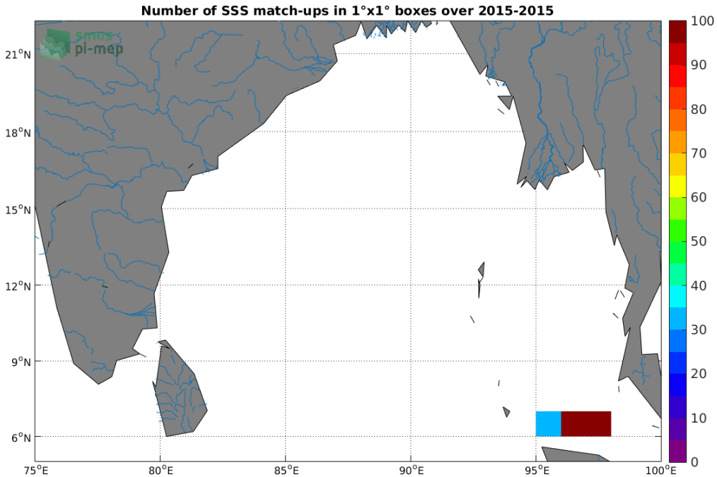
Figure 4: Number of SSS match-ups between TSG (SAMOS) SSS and the SMOS SSS L2 v662 (ESA) SSS product for the Ganga and Brahmaputra river plumes Pi-MEP region over 1°x1° boxes and for the full satellite product period.
