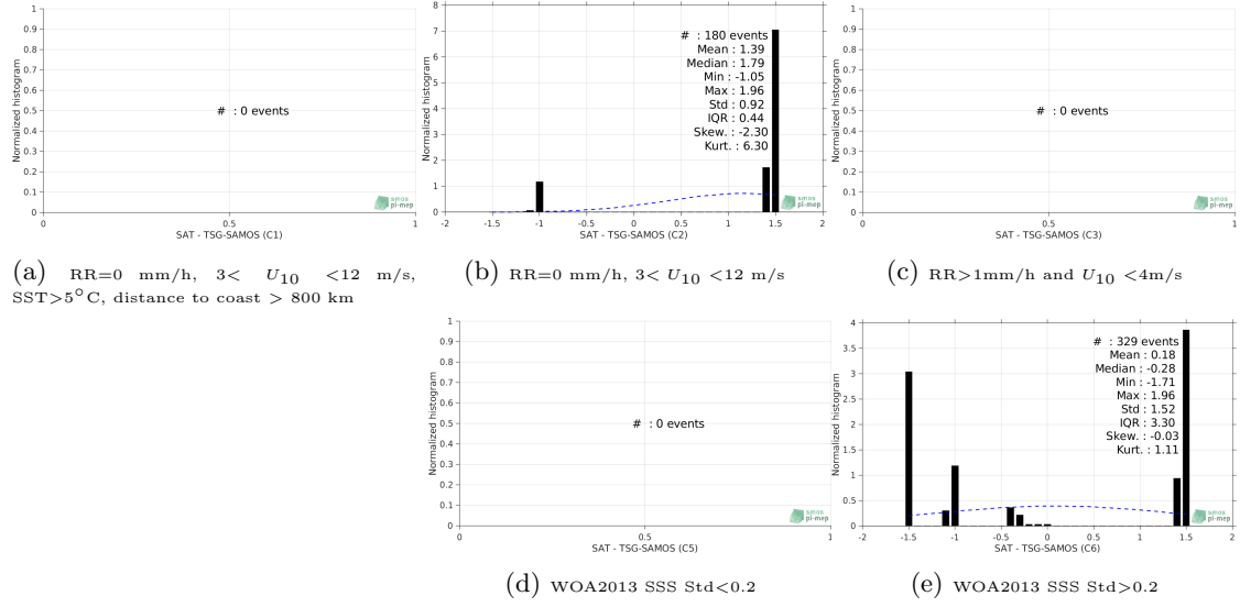
Figure 13: Normalized histogram of \Delta\text{SSS} (SMOS-L2-DPGS-v662 - TSG-SAMOS) for 5 different subdatasets corresponding to: RR=0 mm/h, 3 < U_{10} < 12 m/s, SST > 5^\circ\text{C} , distance to coast > 800 km (a), RR=0 mm/h, 3 < U_{10} < 12 m/s (b), RR > 1\text{mm/h} and U_{10} < 4\text{m/s} (c), WOA2013 SSS Std < 0.2 (d), WOA2013 SSS Std > 0.2 (e).
