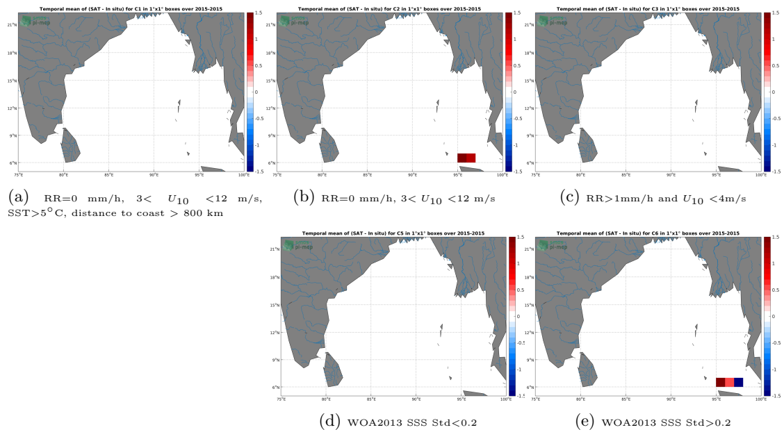
Figure 12: Temporal mean gridded over spatial boxes of size 1^\circ \times 1^\circ of \Delta SSS (SMOS-L2-DPGS-v662 - TSG-SAMOS) for 5 different subdatasets corresponding to:RR=0 mm/h, 3 < U_{10} < 12 m/s, SST >5^\circ C, distance to coast > 800 km (a), RR=0 mm/h, 3 < U_{10} < 12 m/s (b), RR >1 mm/h and U_{10} < 4 m/s (c), WOA2013 SSS Std <0.2 (d), WOA2013 SSS Std >0.2 (e).
