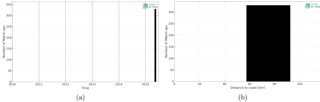
Figure 1: Number of match-ups between TSG-SAMOS and SMOS-L2-DPGS-v662 SSS as a function of time (a) and as function of the distance to coast (b) over the Ganga and Brahmaputra river plumes Pi-MEP region and for the full satellite product period.
