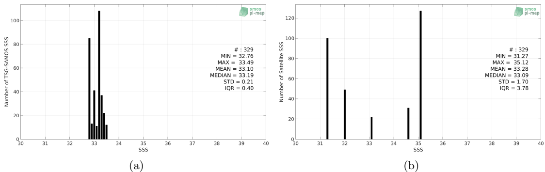
Figure 2: Histograms of SSS from TSG-SAMOS (a) and SMOS-L2-DPGS-v662 (b) considering all match-up pairs per bins of 0.1 over the Ganga and Brahmaputra river plumes Pi-MEP region and for the full satellite product period.
