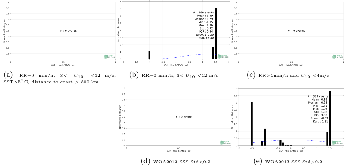
Figure 13: Normalized histogram of \Delta SSS (SMOS-L2-DPGS-v662 - TSG-SAMOS) for 5 different subdatasets corresponding to: RR=0 mm/h, 3 < U_{10} < 12 m/s, SST > 5°C, distance to coast > 800 km (a), RR=0 mm/h, 3 < U_{10} < 12 m/s (b), RR > 1mm/h and U_{10} < 4 m/s (c), WOA2013 SSS Std < 0.2 (d), WOA2013 SSS Std > 0.2 (e).
