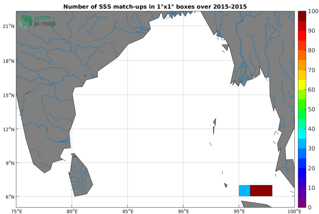
Figure 4: Number of SSS match-ups between TSG-SAMOS SSS and the SMOS-L2-DPGS-v662 SSS product for the Ganga and Brahmaputra river plumes Pi-MEP region over 1^\circ \times 1^\circ boxes and for the full satellite product period.
