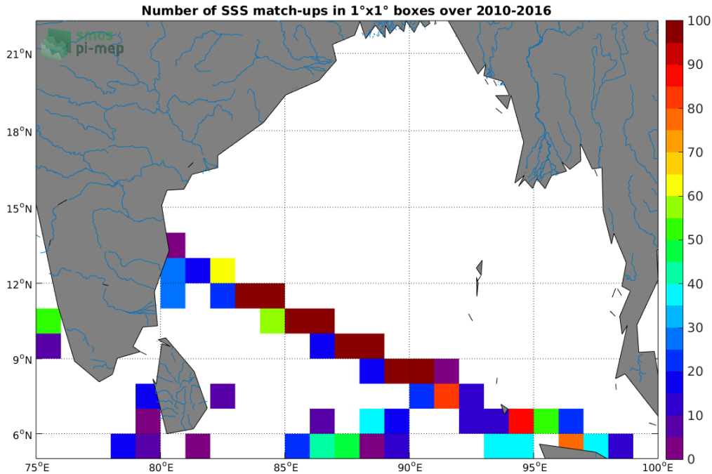
Figure 4: Number of SSS match-ups between TSG (LEGOS-DM) SSS and the SMOS SSS L2 v662 (ESA) SSS product for the Ganga and Brahmaputra river plumes Pi-MEP region over 1°x1° boxes and for the full satellite product period.
