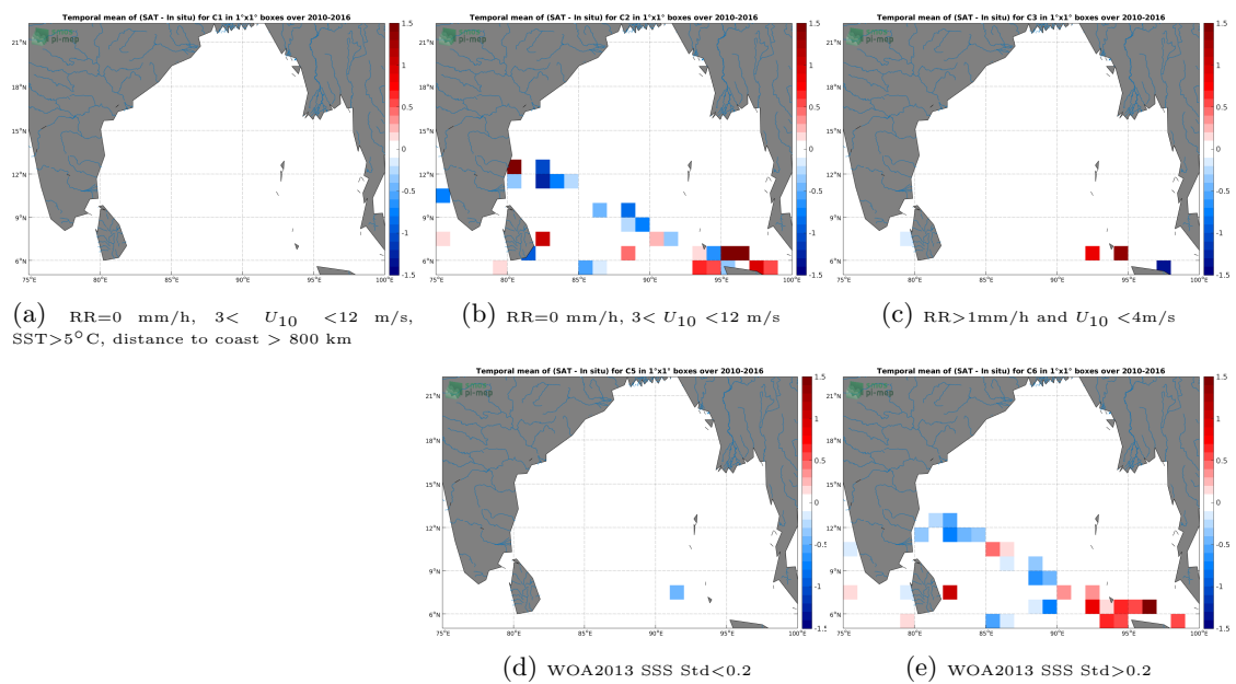
Figure 12: Temporal mean gridded over spatial boxes of size 1°x1° of \Delta SSS (SMOS SSS L2 v662 (ESA) - TSG (LEGOS-DM)) for 5 different subdatasets corresponding to:RR=0 mm/h, 3 < U_{10} < 12 m/s, SST>5°C, distance to coast > 800 km (a), RR=0 mm/h, 3 < U_{10} < 12 m/s (b), RR>1mm/h and U_{10} < 4 m/s (c), WOA2013 SSS Std<0.2 (d), WOA2013 SSS Std>0.2 (e).
