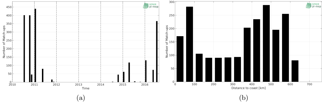
Figure 1: Number of match-ups between TSG-LEGOS-DM and SMOS L2 v662 (ESA) SSS as a function of time (a) and as function of the distance to coast (b) over the Ganga and Brahmaputra river plumes Pi-MEP region and for the full satellite product period.
