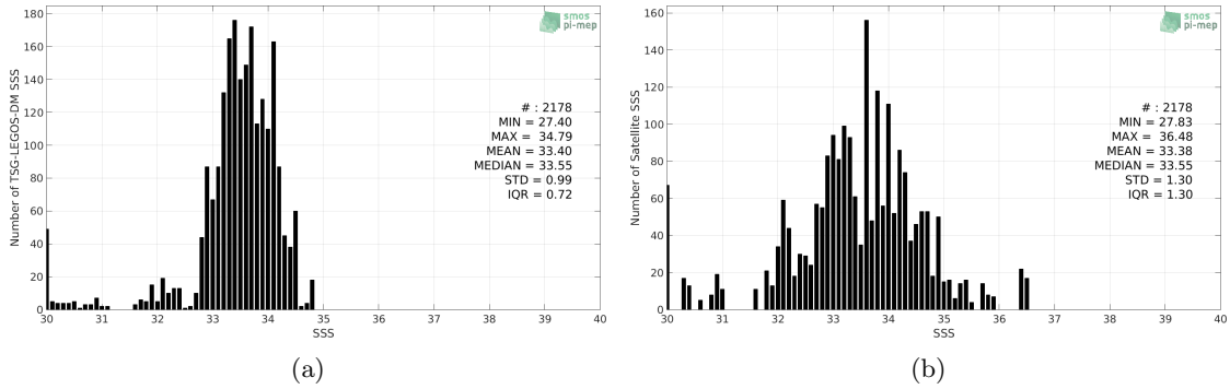
Figure 2: Histograms of SSS from TSG-LEGOS-DM (a) and SMOS L2 v662 (ESA) (b) considering all match-up pairs per bins of 0.1 over the Ganga and Brahmaputra river plumes Pi-MEP region and for the full satellite product period.
