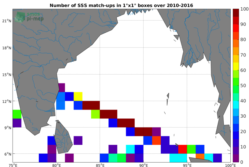
Figure 4: Number of SSS match-ups between TSG-LEGOS-DM SSS and the SMOS L2 v662 (ESA) SSS product for the Ganga and Brahmaputra river plumes Pi-MEP region over 1^\circ \times 1^\circ boxes and for the full satellite product period.
