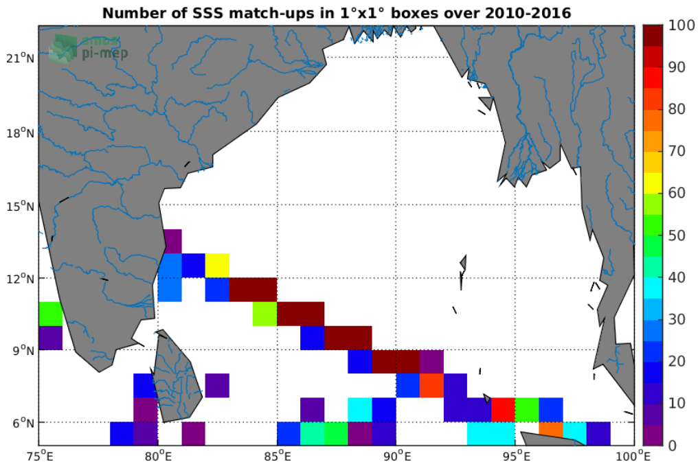
Figure 4: Number of SSS match-ups between TSG-LEGOS-DM SSS and the SMOS-L2-DPGS-v662 SSS product for the Ganga and Brahmaputra river plumes Pi-MEP region over 1^\circ \times 1^\circ boxes and for the full satellite product period.
