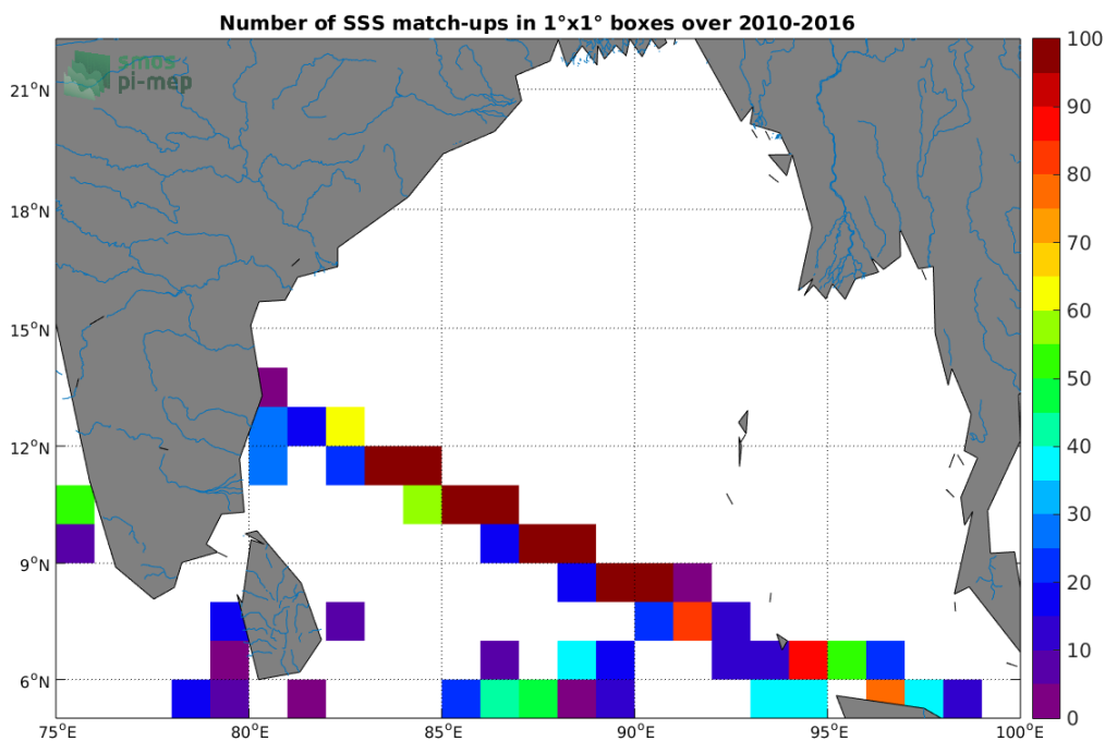
Figure 4: Number of SSS match-ups between TSG-LEGOS-DM SSS and the SMOS-L2-DPGS-v662 SSS product for the Ganga and Brahmaputra river plumes Pi-MEP region over 1^{\circ} \times 1^{\circ} boxes and for the full satellite product period.
