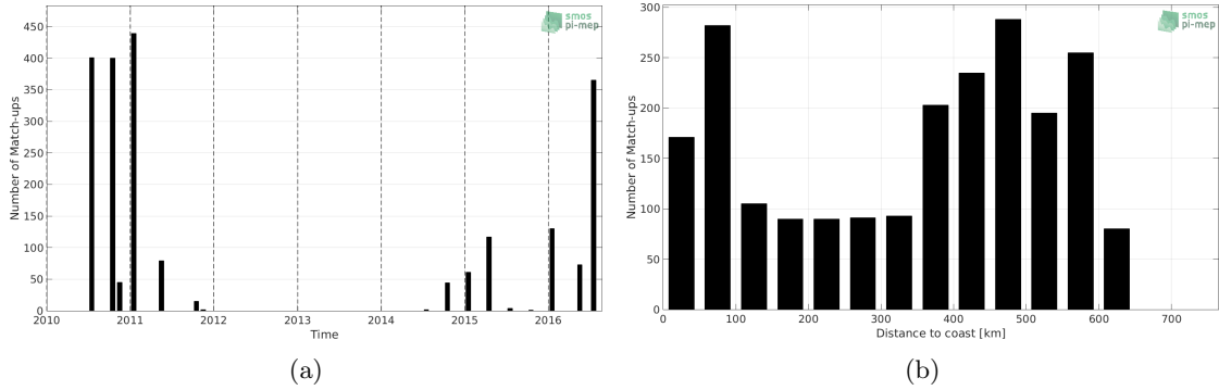
Figure 1: Number of match-ups between TSG-LEGOS-DM and SMOS-L2-DPGS-v662 SSS as a function of time (a) and as function of the distance to coast (b) over the Ganga and Brahmaputra river plumes Pi-MEP region and for the full satellite product period.
