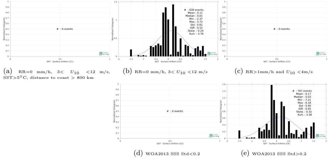
Figure 12: Normalized histogram of \Delta\text{SSS} (SMOS SSS L2 v662 (ESA) - Surface drifters) for 5 different subdatasets corresponding to: RR=0 mm/h, 3 < U_{10} < 12 m/s, SST > 5^\circ\text{C} , distance to coast > 800 km (a), RR=0 mm/h, 3 < U_{10} < 12 m/s (b), RR > 1\text{mm/h} and U_{10} < 4\text{m/s} (c), WOA2013 SSS Std < 0.2 (d), WOA2013 SSS Std > 0.2 (e).
