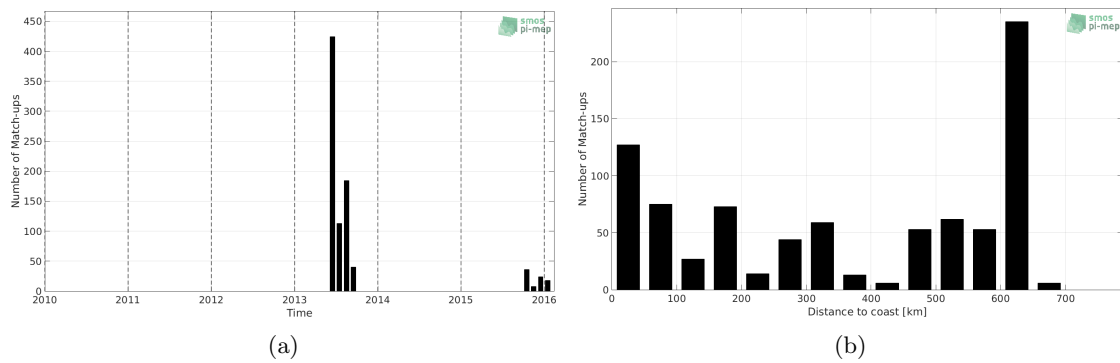
Figure 1: Number of match-ups between Surface drifters and SMOS SSS L2 v662 (ESA) SSS as a function of time (a) and as function of the distance to coast (b) over the Ganga and Brahmaputra river plumes Pi-MEP region and for the full satellite product period.
