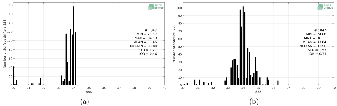
Figure 2: Histograms of SSS from Surface drifters (a) and SMOS SSS L2 v662 (ESA) (b) considering all match-up pairs per bins of 0.1 over the Ganga and Brahmaputra river plumes Pi-MEP region and for the full satellite product period.
