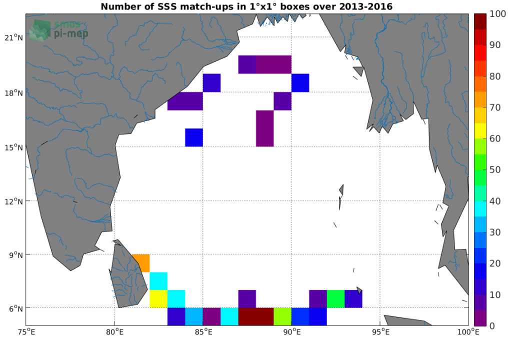
Figure 3: Number of SSS match-ups between Surface drifters SSS and the SMOS SSS L2 v662 (ESA) SSS product for the Ganga and Brahmaputra river plumes Pi-MEP region over 1°x1° boxes and for the full satellite product period.
