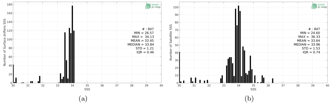
Figure 2: Histograms of SSS from Surface drifters (a) and SMOS L2 v662 (ESA) (b) considering all match-up pairs per bins of 0.1 over the Ganga and Brahmaputra river plumes Pi-MEP region and for the full satellite product period.
