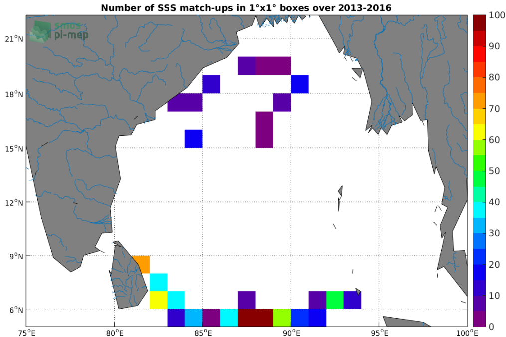
Figure 3: Number of SSS match-ups between Surface drifters SSS and the SMOS-L2-DPGS-v662 SSS product for the Ganga and Brahmaputra river plumes Pi-MEP region over 1°x1° boxes and for the full satellite product period.
