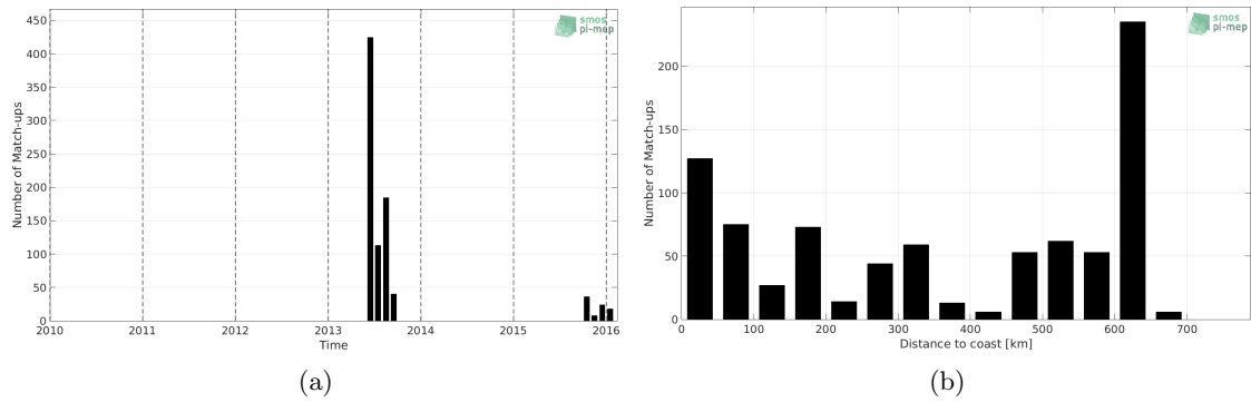
Figure 1: Number of match-ups between Surface drifters and SMOS-L2-DPGS-v662 SSS as a function of time (a) and as function of the distance to coast (b) over the Ganga and Brahmaputra river plumes Pi-MEP region and for the full satellite product period.
