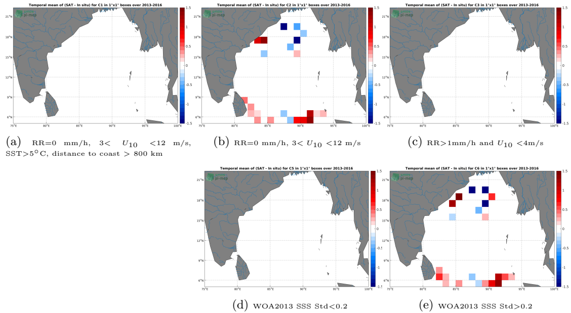
Figure 11: Temporal mean gridded over spatial boxes of size 1^\circ \times 1^\circ of \Delta SSS (SMOS-L2-DPGS-v662 - Surface drifters) for 5 different subdatasets corresponding to:RR=0 mm/h, 3 < U_{10} < 12 m/s, SST >5^\circ C, distance to coast > 800 km (a), RR=0 mm/h, 3 < U_{10} < 12 m/s (b), RR >1 mm/h and U_{10} < 4 m/s (c), WOA2013 SSS Std <0.2 (d), WOA2013 SSS Std >0.2 (e).
