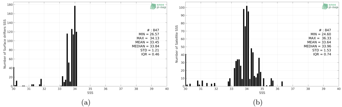
Figure 2: Histograms of SSS from Surface drifters (a) and SMOS-L2-DPGS-v662 (b) considering all match-up pairs per bins of 0.1 over the Ganga and Brahmaputra river plumes Pi-MEP region and for the full satellite product period.
