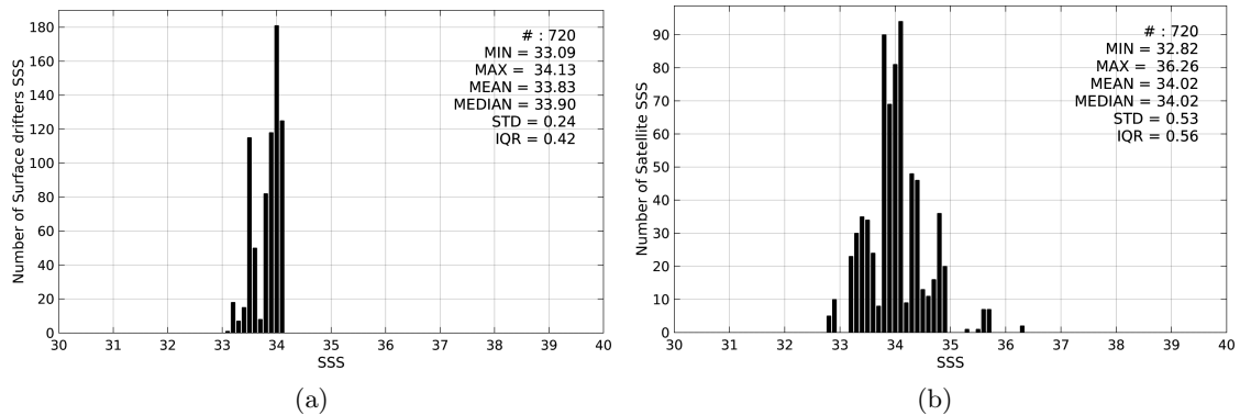
Figure 2: Histograms of SSS from Surface drifters (a) and SMOS-L2-DPGS-v662 (b) considering all match-up pairs per bins of 0.1 over the Ganga and Brahmaputra river plumes Pi-MEP region and for the full satellite product period.
