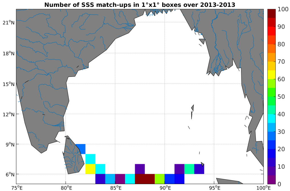
Figure 3: Number of SSS match-ups between Surface drifters SSS and the SMOS-L2-DPGS-v662 SSS product for the Ganga and Brahmaputra river plumes Pi-MEP region over 1^{\circ} \times 1^{\circ} boxes and for the full satellite product period.
