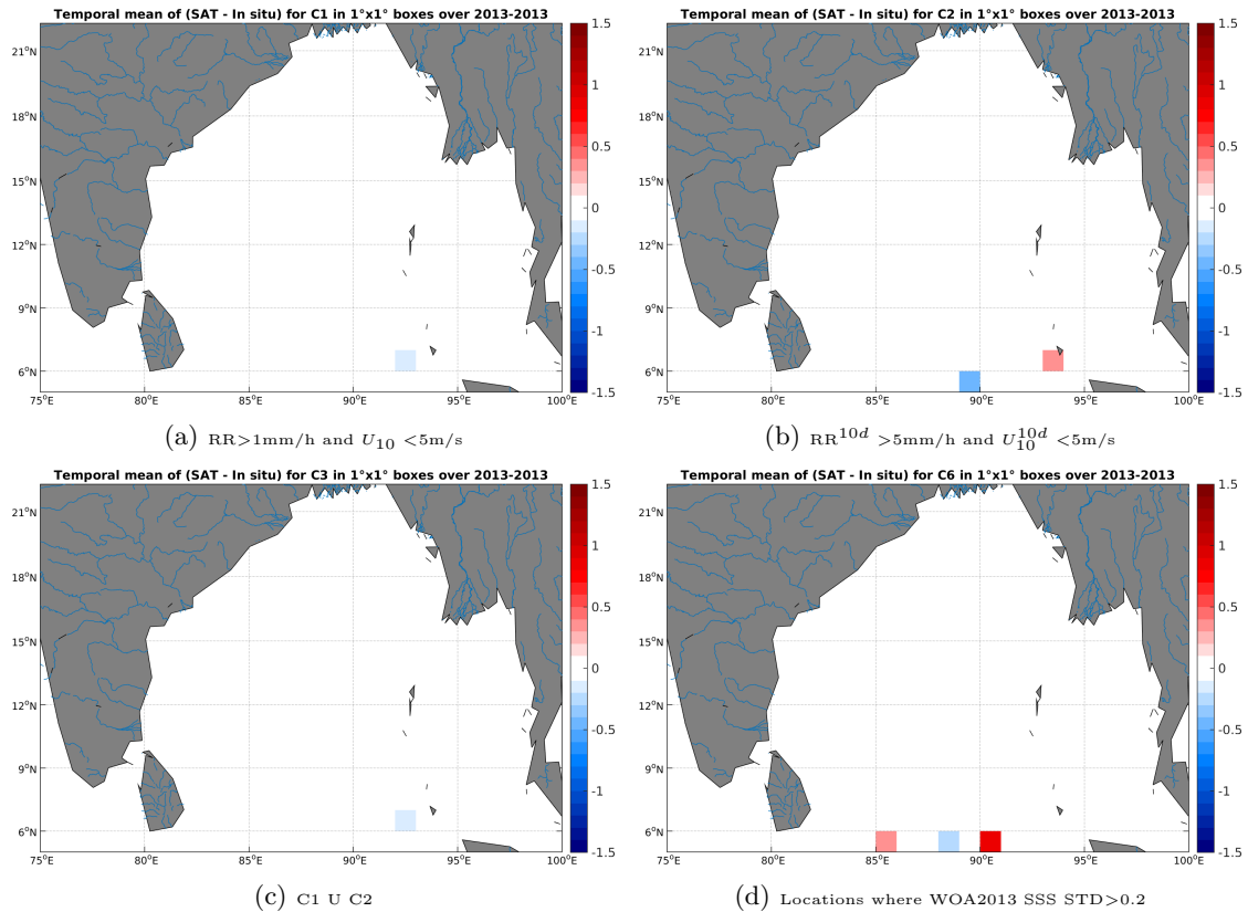
Figure 11: Temporal mean gridded over spatial boxes of size 1^\circ \times 1^\circ of \Delta SSS (SMOS-L2-DPGS-v662 - Surface drifters) for 4 different subdatasets corresponding to: RR > 1mm/h and U_{10} < 5 m/s (a), RR^{10d} > 5 mm/h and U_{10}^{10d} < 5 m/s (b), C1 U C2 (c), Locations where WOA2013 SSS STD > 0.2 (d).
