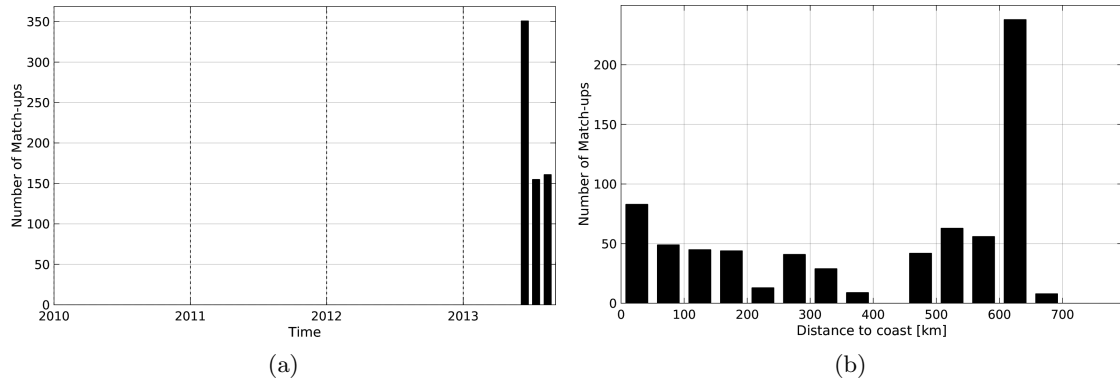
Figure 1: Number of match-ups between Surface drifters and SMOS-L2-DPGS-v662 SSS as a function of time (a) and as function of the distance to coast (b) over the Ganga and Brahmaputra river plumes Pi-MEP region and for the full satellite product period.
