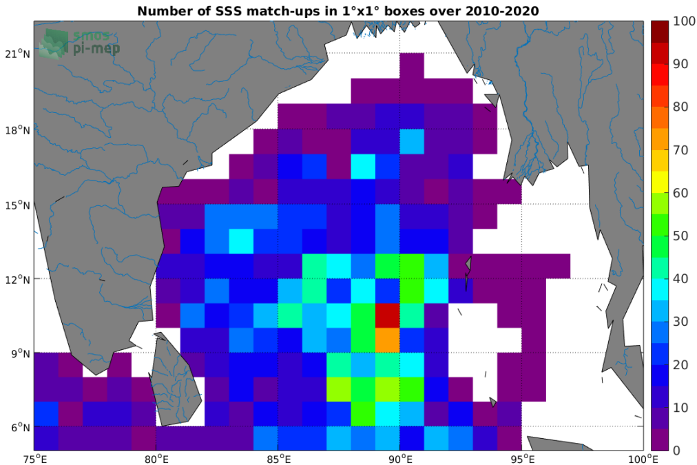
Figure 4: Number of SSS match-ups between Argos SSS and the SMOS L2 v662 (ESA) SSS product for the Ganga and Brahmaputra river plumes Pi-MEP region over 1°x1° boxes and for the full satellite product period.
