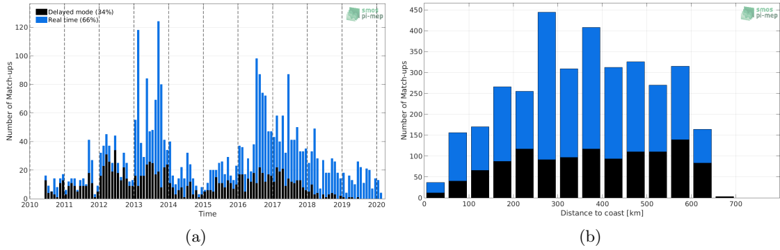
Figure 1: Number of match-ups between Argo and SMOS L2 v662 (ESA) SSS as a function of time (a) and as function of the distance to coast (b) over the Ganga and Brahmaputra river plumes Pi-MEP region and for the full satellite product period.
