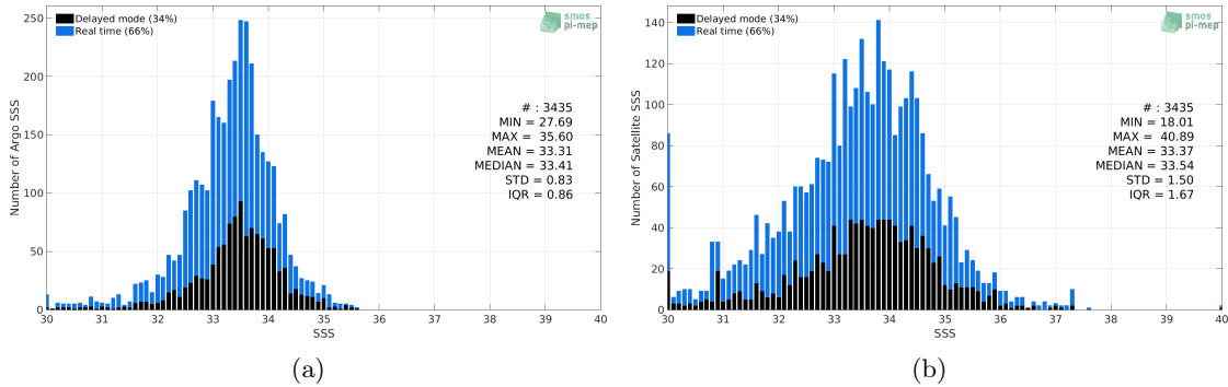
Figure 2: Histograms of SSS from Argo (a) and SMOS L2 v662 (ESA) (b) considering all match-up pairs per bins of 0.1 over the Ganga and Brahmaputra river plumes Pi-MEP region and for the full satellite product period.
