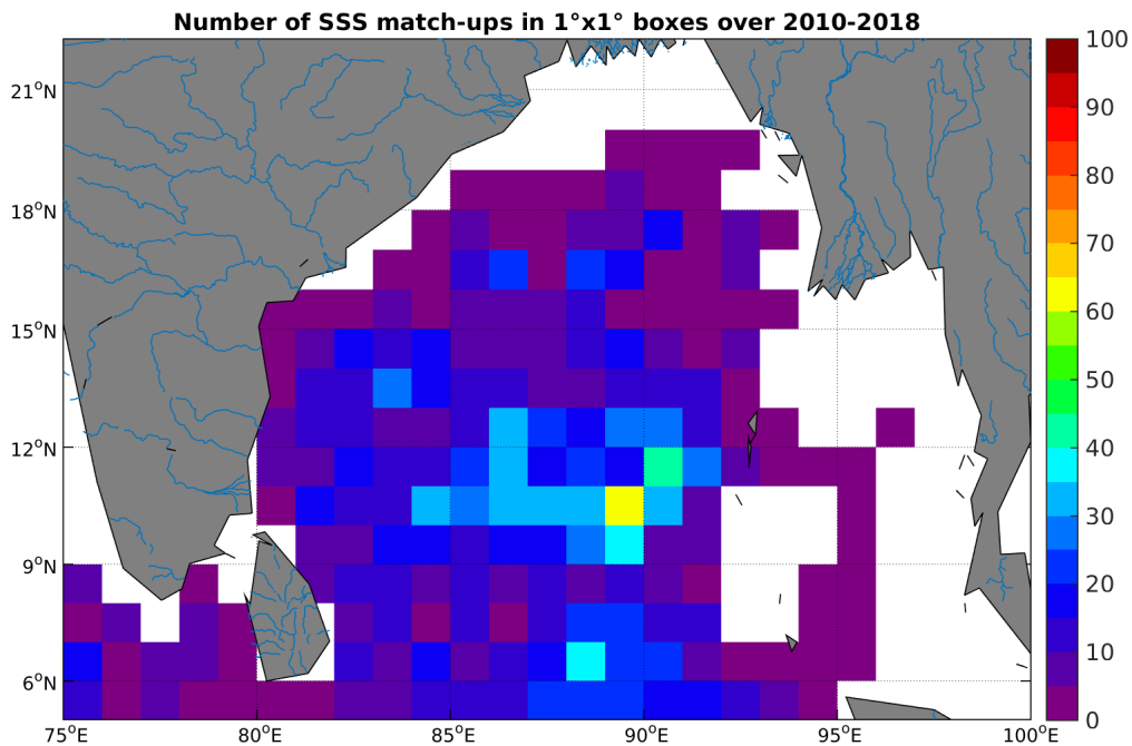
Figure 4: Number of SSS match-ups between Argo SSS and the SMOS-L2-DPGS-v662 SSS product for the Ganga and Brahmaputra river plumes Pi-MEP region over 1^\circ \times 1^\circ boxes and for the full satellite product period.
