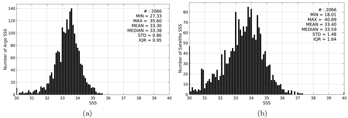
Figure 2: Histograms of SSS from Argo (a) and SMOS-L2-DPGS-v662 (b) considering all match-up pairs per bins of 0.1 over the Ganga and Brahmaputra river plumes Pi-MEP region and for the full satellite product period.
