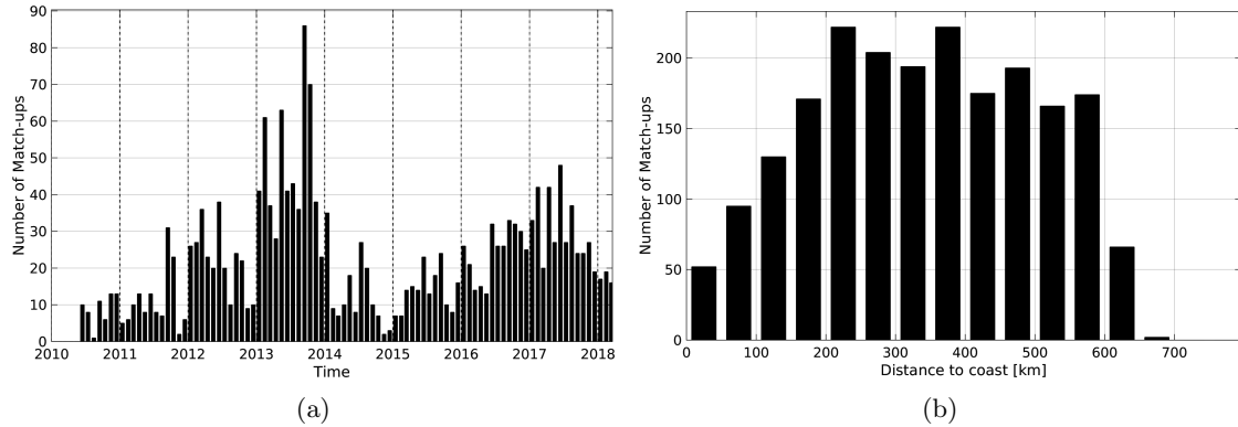
Figure 1: Number of match-ups between Argo and SMOS-L2-DPGS-v662 SSS as a function of time (a) and as function of the distance to coast (b) over the Ganga and Brahmaputra river plumes Pi-MEP region and for the full satellite product period.
