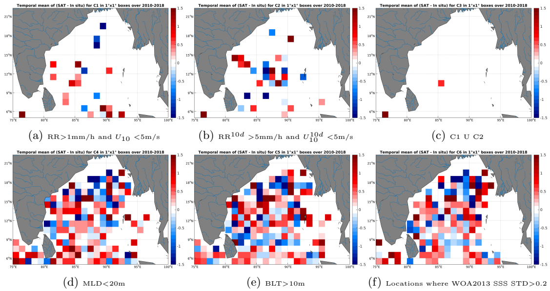
Figure 12: Temporal mean gridded over spatial boxes of size 1^\circ \times 1^\circ of \Delta SSS (SMOS-L2-DPGS-v662 - Argo) for 6 different subdatasets corresponding to: RR > 1\text{mm/h} and U_{10} < 5\text{m/s} (a), RR^{10d} > 5\text{mm/h} and U_{10}^{10d} < 5\text{m/s} (b), C1 U C2 (c), MLD < 20\text{m} (d), BLT > 10\text{m} (e), Locations where WOA2013 SSS STD > 0.2 (f).
