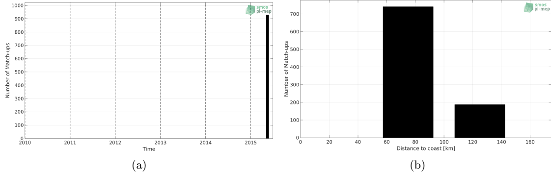
Figure 1: Number of match-ups between TSG (SAMOS) and SMAP SSS L4 OI v1 - 7 Days (IPRC) SSS as a function of time (a) and as function of the distance to coast (b) over the Ganga and Brahmaputra river plumes Pi-MEP region and for the full satellite product period.
