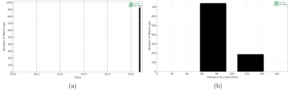
Figure 1: Number of match-ups between TSG (SAMOS) and SMAP SSS L4 OI v1 - 7day (IPRC) SSS as a function of time (a) and as function of the distance to coast (b) over the Ganga and Brahmaputra river plumes Pi-MEP region and for the full satellite product period.
