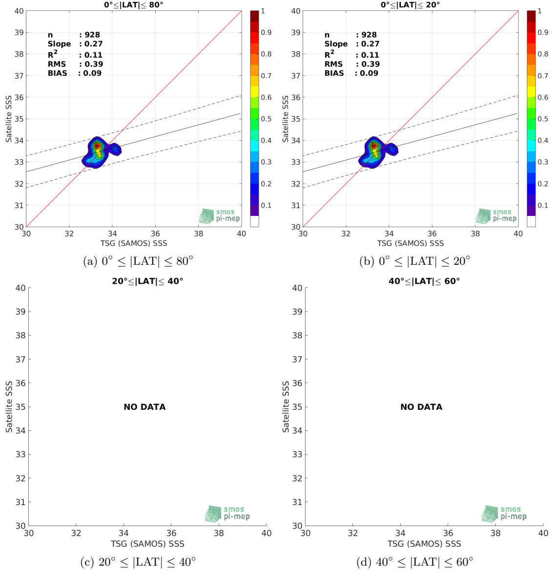
Figure 9: Contour maps of the concentration of SMAP SSS L4 OI v1 - 7day (IPRC) SSS (y-axis) versus TSG (SAMOS) SSS (x-axis) at match-up pairs for different latitude bands. For each plot, the red line shows x=y . The black thin and dashed lines indicate a linear fit through the data cloud and the \pm 95\% confidence levels, respectively. The number match-up pairs n , the slope and R^2 coefficient of the linear fit, the root mean square (RMS) and the mean bias between satellite and in situ data are indicated for each latitude band in each plots.
