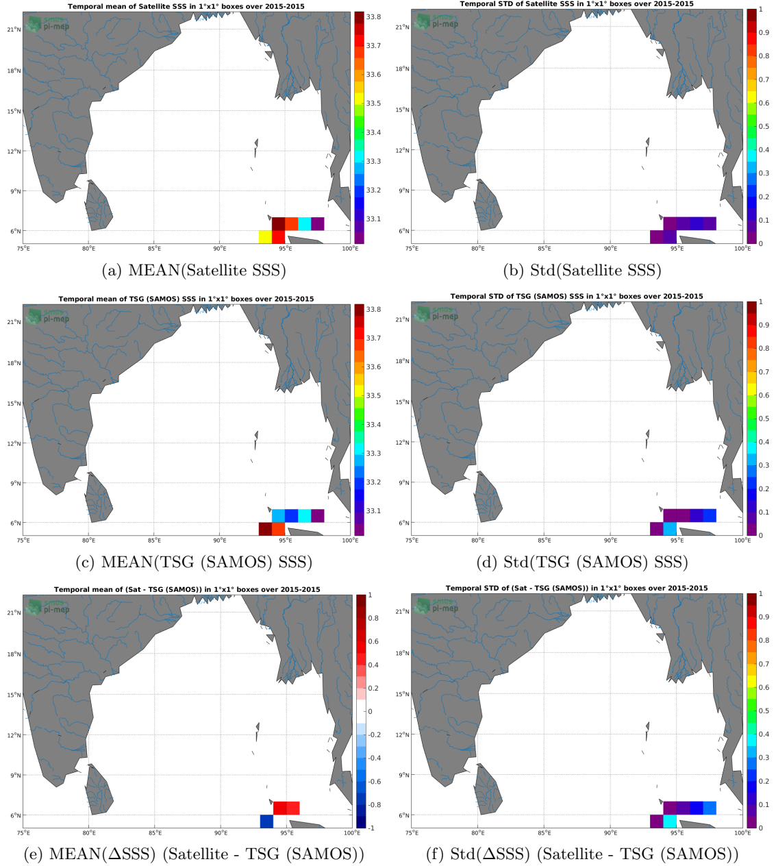
Figure 6: Temporal mean (left) and Std (right) of SSS from SMAP SSS L4 OI v1 - 7day (IPRC) (top), TSG (SAMOS) (middle), and of \Delta SSS (Satellite - TSG (SAMOS)). Only match-up pairs are used to generate these maps.
