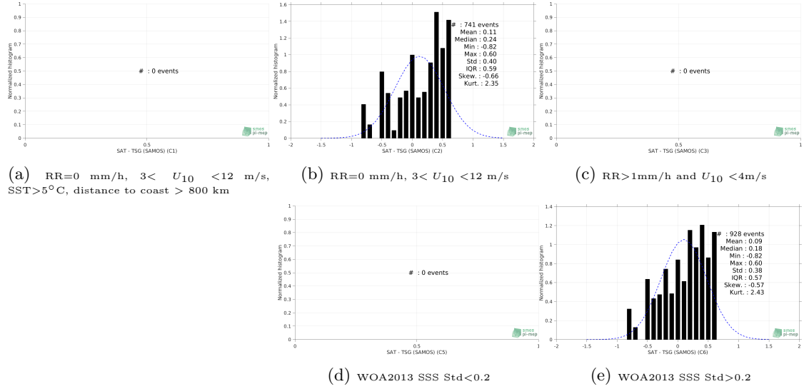
Figure 13: Normalized histogram of \Delta\text{SSS} (SMAP SSS L4 OI v1 - 7day (IPRC) - TSG (SAMOS)) for 5 different subdatasets corresponding to: RR=0 mm/h, 3 < U_{10} < 12 m/s, SST > 5^\circ\text{C} , distance to coast > 800 km (a), RR=0 mm/h, 3 < U_{10} < 12 m/s (b), RR > 1 mm/h and U_{10} < 4 m/s (c), WOA2013 SSS Std < 0.2 (d), WOA2013 SSS Std > 0.2 (e).
