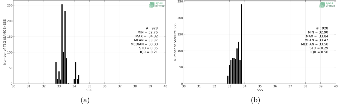
Figure 2: Histograms of SSS from TSG (SAMOS) (a) and SMAP SSS L4 OI v1 - 7day (IPRC) (b) considering all match-up pairs per bins of 0.1 over the Ganga and Brahmaputra river plumes Pi-MEP region and for the full satellite product period.
