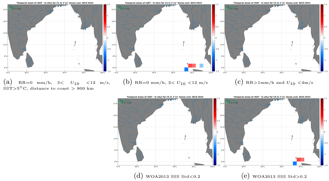
Figure 12: Temporal mean gridded over spatial boxes of size 1^\circ \times 1^\circ of \Delta SSS (SMAP SSS L4 OI v1 - 7day (IPRC) - TSG (SAMOS)) for 5 different subdatasets corresponding to:RR=0 mm/h, 3 < U_{10} < 12 m/s, SST>5°C, distance to coast > 800 km (a), RR=0 mm/h, 3 < U_{10} < 12 m/s (b), RR>1mm/h and U_{10} < 4 m/s (c), WOA2013 SSS Std<0.2 (d), WOA2013 SSS Std>0.2 (e).
