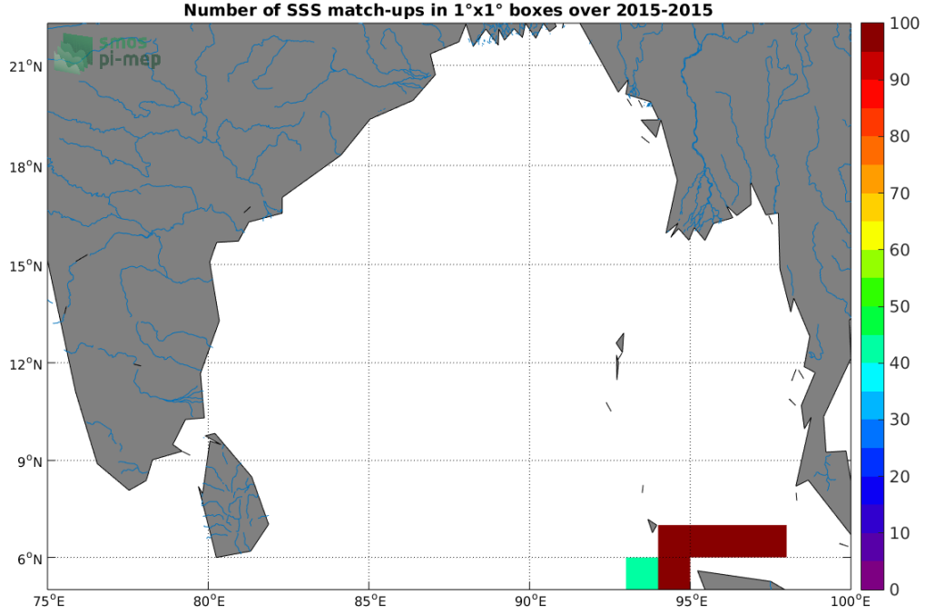
Figure 4: Number of SSS match-ups between TSG (SAMOS) SSS and the SMAP SSS L4 OI v1 - 7day (IPRC) SSS product for the Ganga and Brahmaputra river plumes Pi-MEP region over 1^\circ \times 1^\circ boxes and for the full satellite product period.
