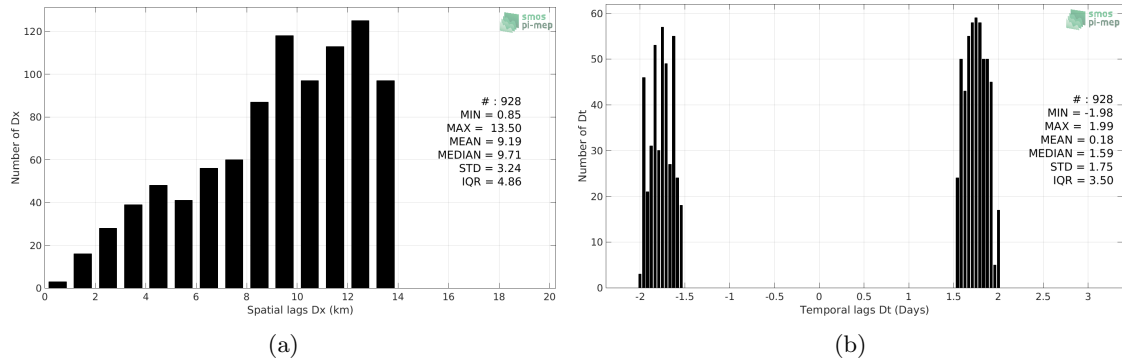
Figure 5: Histograms of the spatial (a) and temporal (b) lags between the location/time of the TSG (SAMOS) measurement and the date of the corresponding SMAP SSS L4 OI v1 - 7day (IPRC) SSS pixel.
