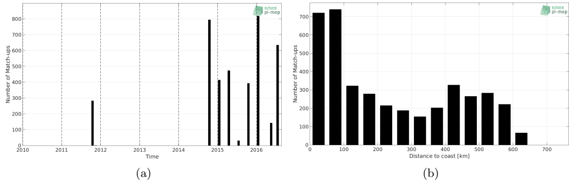
Figure 1: Number of match-ups between TSG (LEGOS-DM) and SMAP SSS L4 OI v1 - 7 Days (IPRC) SSS as a function of time (a) and as function of the distance to coast (b) over the Ganga and Brahmaputra river plumes Pi-MEP region and for the full satellite product period.
