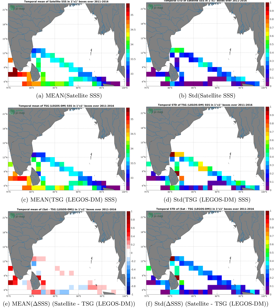
Figure 6: Temporal mean (left) and Std (right) of SSS from SMAP SSS L4 OI v1 - 7 Days (IPRC) (top), TSG (LEGOS-DM) (middle), and of \Delta SSS (Satellite - TSG (LEGOS-DM)). Only match-up pairs are used to generate these maps.
