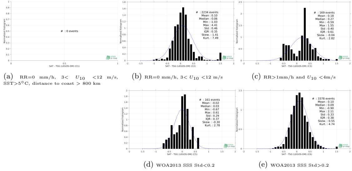
Figure 13: Normalized histogram of \Delta SSS (SMAP SSS L4 OI v1 - 7 Days (IPRC) - TSG (LEGOS-DM)) for 5 different subdatasets corresponding to: RR=0 mm/h, 3 < U_{10} < 12 m/s, SST>5°C, distance to coast > 800 km (a), RR=0 mm/h, 3 < U_{10} < 12 m/s (b), RR>1mm/h and U_{10} < 4 m/s (c), WOA2013 SSS Std<0.2 (d), WOA2013 SSS Std>0.2 (e).
