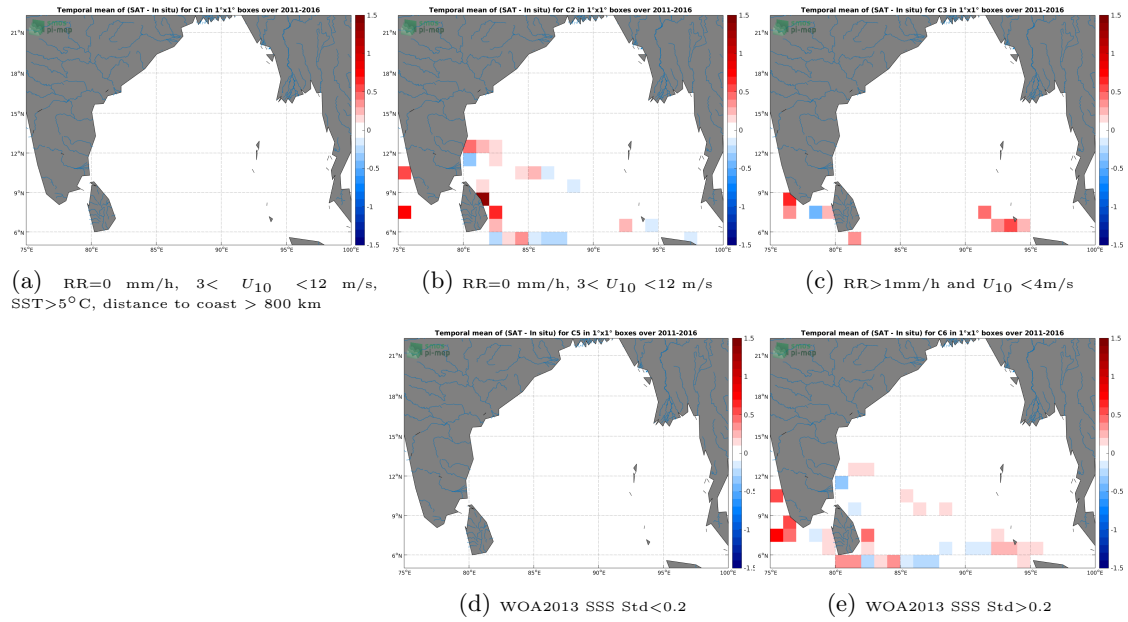
Figure 12: Temporal mean gridded over spatial boxes of size 1^\circ \times 1^\circ of \Delta SSS (SMAP SSS L4 OI v1 - 7 Days (IPRC) - TSG (LEGOS-DM)) for 5 different subdatasets corresponding to: RR=0 mm/h, 3 < U_{10} < 12 m/s, SST >5^\circ\text{C} , distance to coast > 800 km (a), RR=0 mm/h, 3 < U_{10} < 12 m/s (b), RR >1 mm/h and U_{10} < 4 m/s (c), WOA2013 SSS Std <0.2 (d), WOA2013 SSS Std >0.2 (e).
