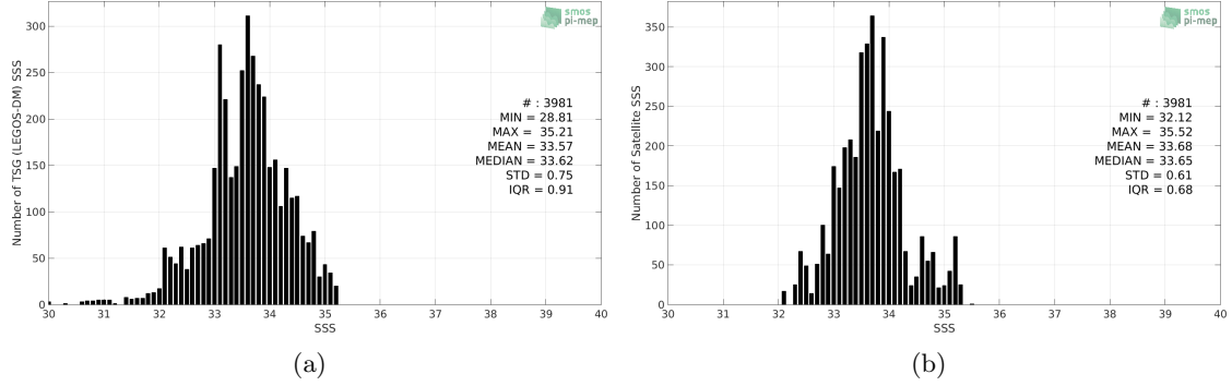
Figure 2: Histograms of SSS from TSG (LEGOS-DM) (a) and SMAP SSS L4 OI v1 - 7 Days (IPRC) (b) considering all match-up pairs per bins of 0.1 over the Ganga and Brahmaputra river plumes Pi-MEP region and for the full satellite product period.
