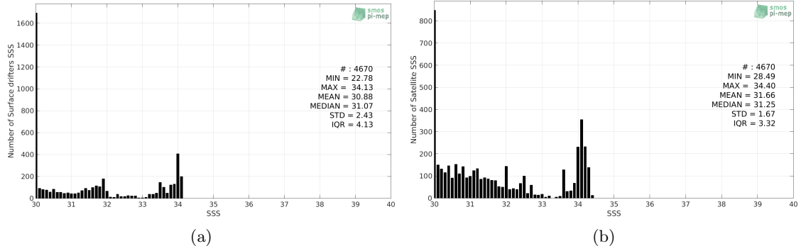
Figure 2: Histograms of SSS from Surface drifters (a) and SMAP SSS L4 OI v1 - 7 Days (IPRC) (b) considering all match-up pairs per bins of 0.1 over the Ganga and Brahmaputra river plumes Pi-MEP region and for the full satellite product period.
