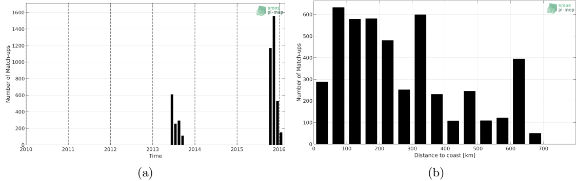
Figure 1: Number of match-ups between Surface drifters and SMAP SSS L4 OI v1 - 7 Days (IPRC) SSS as a function of time (a) and as function of the distance to coast (b) over the Ganga and Brahmaputra river plumes Pi-MEP region and for the full satellite product period.
