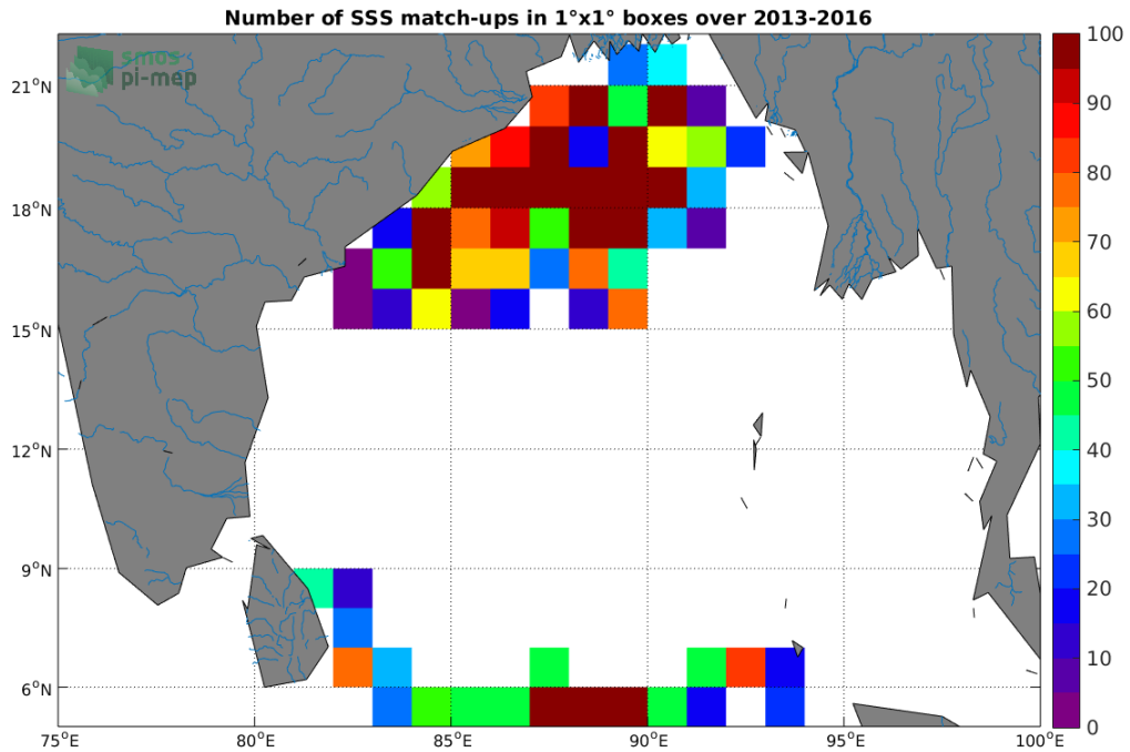
Figure 3: Number of SSS match-ups between Surface drifters SSS and the SMAP SSS L4 OI v1 - 7 Days (IPRC) SSS product for the Ganga and Brahmaputra river plumes Pi-MEP region over 1^\circ \times 1^\circ boxes and for the full satellite product period.
