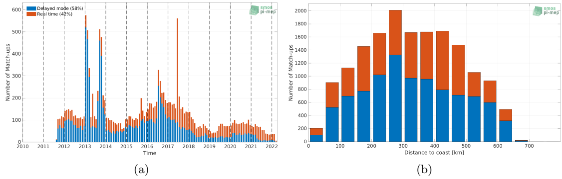
Figure 1: Number of match-ups between Argo and SMAP SSS L4 OI v1 - 7 Days (IPRC) SSS as a function of time (a) and as function of the distance to coast (b) over the Ganga and Brahmaputra river plumes Pi-MEP region and for the full satellite product period.
