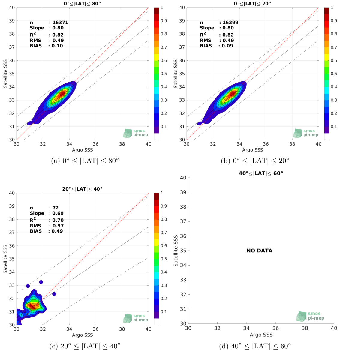
Figure 9: Contour maps of the concentration of SMAP SSS L4 OI v1 - 7 Days (IPRC) SSS (y-axis) versus Argo SSS (x-axis) at match-up pairs for different latitude bands. For each plot, the red line shows x=y . The black thin and dashed lines indicate a linear fit through the data cloud and the \pm 95\% confidence levels, respectively. The number match-up pairs n , the slope and R^2 coefficient of the linear fit, the root mean square (RMS) and the mean bias between satellite and in situ data are indicated for each latitude band in each plots.
