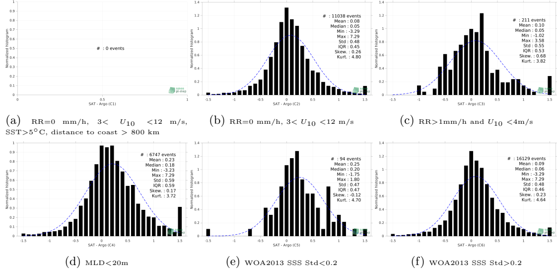
Figure 13: Normalized histogram of \Delta\text{SSS} (SMAP SSS L4 OI v1 - 7 Days (IPRC) - Argo) for 6 different subdatasets corresponding to: RR=0 mm/h, 3 < U_{10} < 12 m/s, SST>5°C, distance to coast > 800 km (a), RR=0 mm/h, 3 < U_{10} < 12 m/s (b), RR>1mm/h and U_{10} < 4 m/s (c), MLD<20m (d), WOA2013 SSS Std<0.2 (e), WOA2013 SSS Std>0.2 (f).
