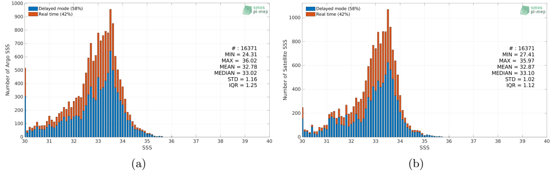
Figure 2: Histograms of SSS from Argo (a) and SMAP SSS L4 OI v1 - 7 Days (IPRC) (b) considering all match-up pairs per bins of 0.1 over the Ganga and Brahmaputra river plumes Pi-MEP region and for the full satellite product period.
