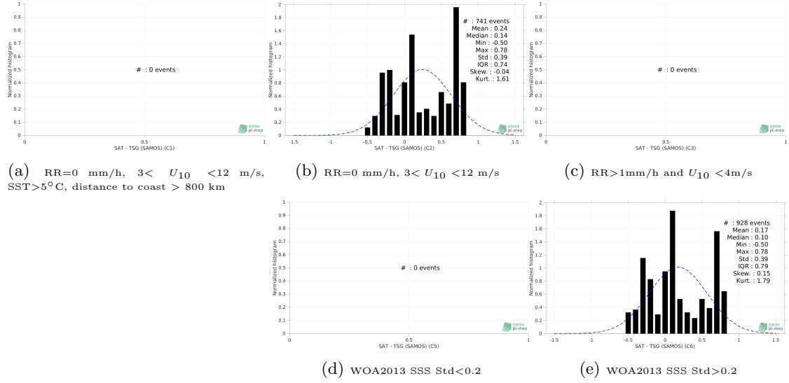
Figure 13: Normalized histogram of \Delta SSS (SMAP SSS L4 OI v1 - Monthly (IPRC) - TSG (SAMOS)) for 5 different subdatasets corresponding to: RR=0 mm/h, 3 < U_{10} < 12 m/s, SST >5^{\circ}\text{C} , distance to coast > 800 km (a), RR=0 mm/h, 3 < U_{10} < 12 m/s (b), RR >1 mm/h and U_{10} < 4 m/s (c), WOA2013 SSS Std <0.2 (d), WOA2013 SSS Std >0.2 (e).
