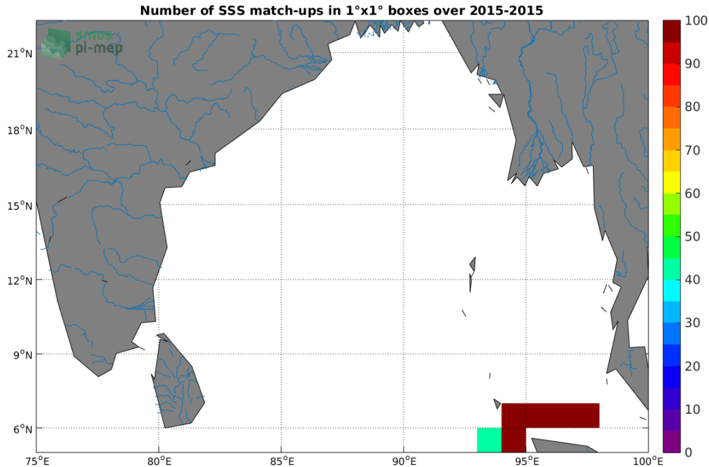
Figure 4: Number of SSS match-ups between TSG (SAMOS) SSS and the SMAP SSS L4 OI v1 - Monthly (IPRC) SSS product for the Ganga and Brahmaputra river plumes Pi-MEP region over 1°x1° boxes and for the full satellite product period.
