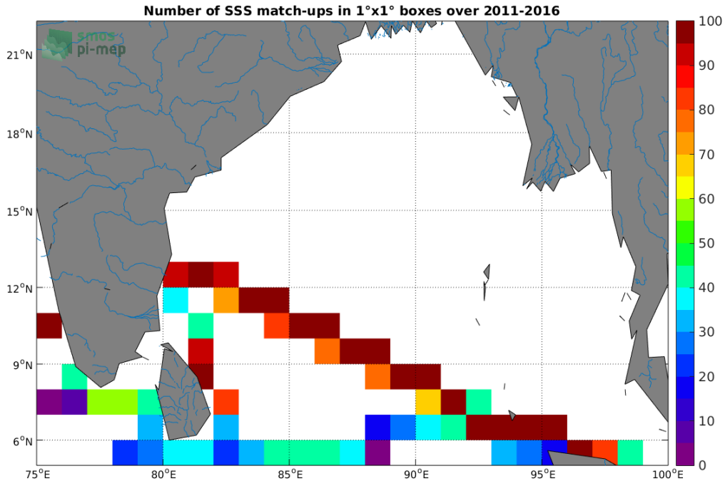
Figure 4: Number of SSS match-ups between TSG (LEGOS-DM) SSS and the SMAP SSS L4 OI v1 - Monthly (IPRC) SSS product for the Ganga and Brahmaputra river plumes Pi-MEP region over 1^{\circ} \times 1^{\circ} boxes and for the full satellite product period.
