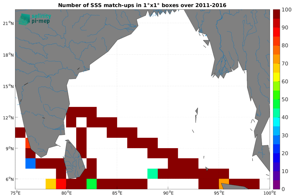
Figure 5: Number of SSS match-ups between TSG (LEGOS-DM) SSS and the SMAP SSS L4 OI v3 - Daily (ESR) SSS product for the Ganga and Brahmaputra river plumes Pi-MEP region over 1^\circ \times 1^\circ boxes and for the full satellite product period.
