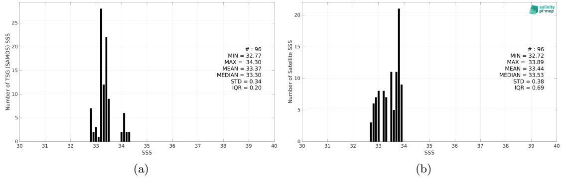
Figure 2: Histograms of SSS from TSG (SAMOS) (a) and SMAP SSS L4 OI v2 - 7 Days (ESR) (b) considering all match-up pairs per bins of 0.1 over the Ganga and Brahmaputra river plumes Pi-MEP region and for the full satellite product period.
