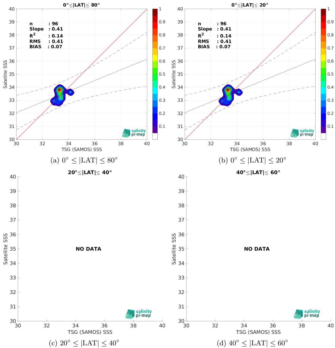
Figure 9: Contour maps of the concentration of SMAP SSS L4 OI v2 - 7 Days (ESR) SSS (y-axis) versus TSG (SAMOS) SSS (x-axis) at match-up pairs for different latitude bands. For each plot, the red line shows x=y . The black thin and dashed lines indicate a linear fit through the data cloud and the \pm 95\% confidence levels, respectively. The number match-up pairs n , the slope and R^2 coefficient of the linear fit, the root mean square (RMS) and the mean bias between satellite and in situ data are indicated for each latitude band in each plots.
