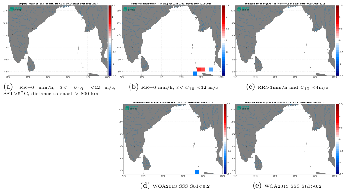
Figure 12: Temporal mean gridded over spatial boxes of size 1^\circ \times 1^\circ of \Delta SSS (SMAP SSS L4 OI v2 - 7 Days (ESR) - TSG (SAMOS)) for 5 different subdatasets corresponding to:RR=0 mm/h, 3 < U_{10} < 12 m/s, SST >5^\circ C, distance to coast > 800 km (a), RR=0 mm/h, 3 < U_{10} < 12 m/s (b), RR >1 mm/h and U_{10} < 4 m/s (c), WOA2013 SSS Std <0.2 (d), WOA2013 SSS Std >0.2 (e).
