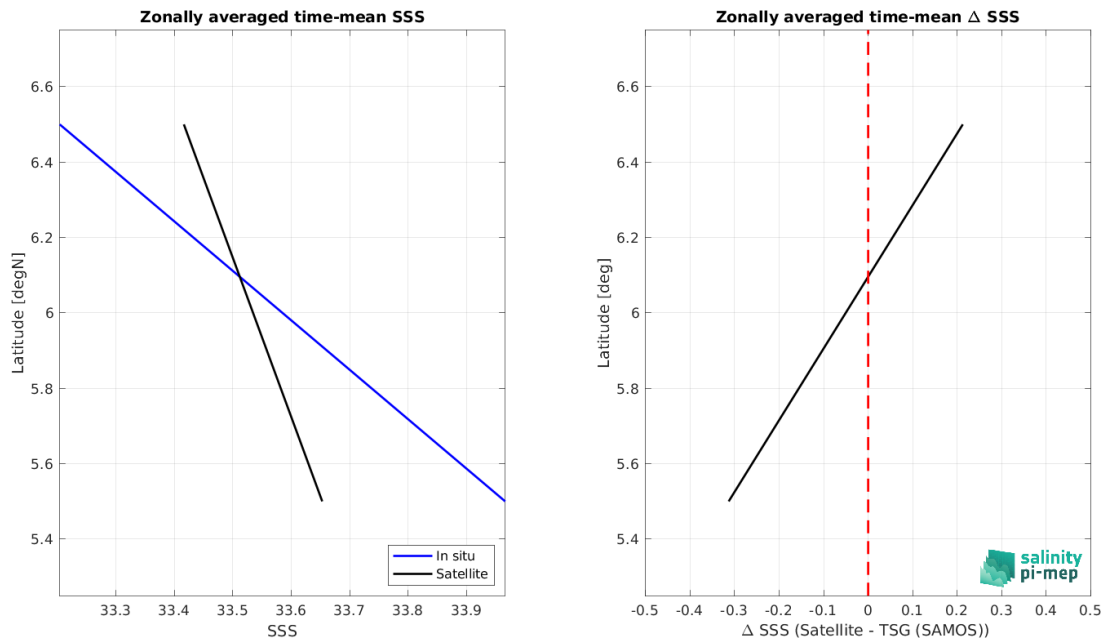
Figure 8: Left panel: Zonal mean SSS from SMAP SSS L4 OI v2 - 7 Days (ESR) satellite product (black) and from TSG (SAMOS) (blue). Right panel: Zonal mean of \Delta SSS (Satellite - TSG (SAMOS)) for all the collected Pi-MEP match-up pairs estimated over the full satellite product period.
