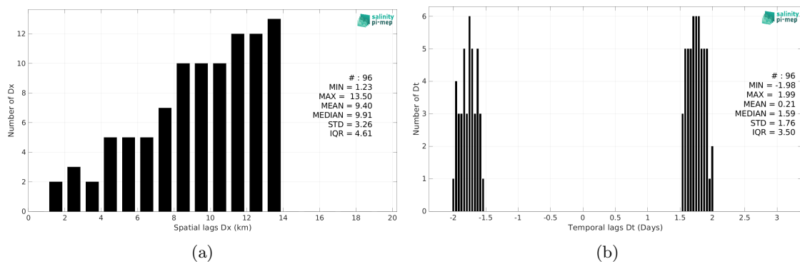
Figure 5: Histograms of the spatial (a) and temporal (b) lags between the location/time of the TSG (SAMOS) measurement and the date of the corresponding SMAP SSS L4 OI v2 - 7 Days (ESR) SSS pixel.
