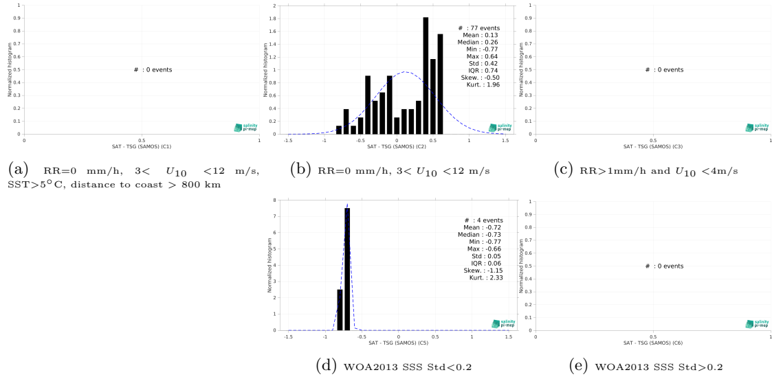
Figure 13: Normalized histogram of \Delta SSS (SMAP SSS L4 OI v2 - 7 Days (ESR) - TSG (SAMOS)) for 5 different subdatasets corresponding to: RR=0 mm/h, 3 < U_{10} < 12 m/s, SST > 5°C, distance to coast > 800 km (a), RR=0 mm/h, 3 < U_{10} < 12 m/s (b), RR > 1mm/h and U_{10} < 4 m/s (c), WOA2013 SSS Std < 0.2 (d), WOA2013 SSS Std > 0.2 (e).
