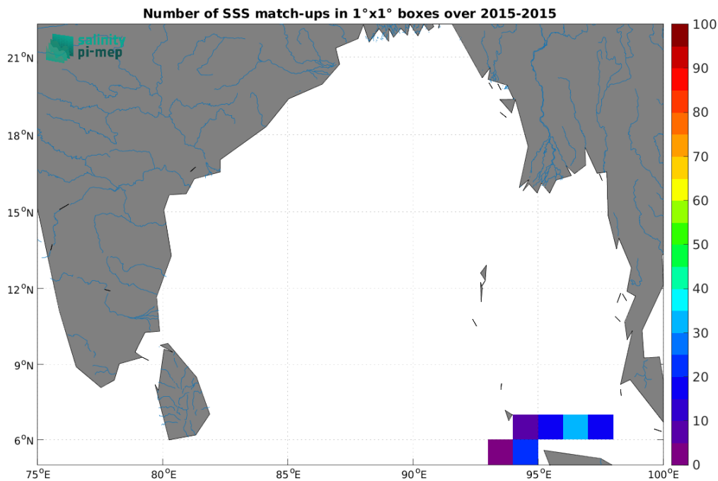
Figure 4: Number of SSS match-ups between TSG (SAMOS) SSS and the SMAP SSS L4 OI v2 - 7 Days (ESR) SSS product for the Ganga and Brahmaputra river plumes Pi-MEP region over 1^\circ \times 1^\circ boxes and for the full satellite product period.
