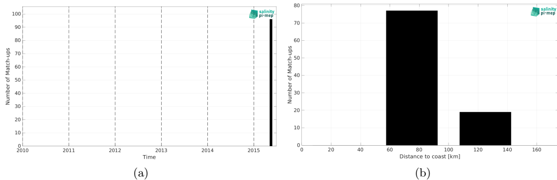
Figure 1: Number of match-ups between TSG (SAMOS) and SMAP SSS L4 OI v2 - 7 Days (ESR) SSS as a function of time (a) and as function of the distance to coast (b) over the Ganga and Brahmaputra river plumes Pi-MEP region and for the full satellite product period.
