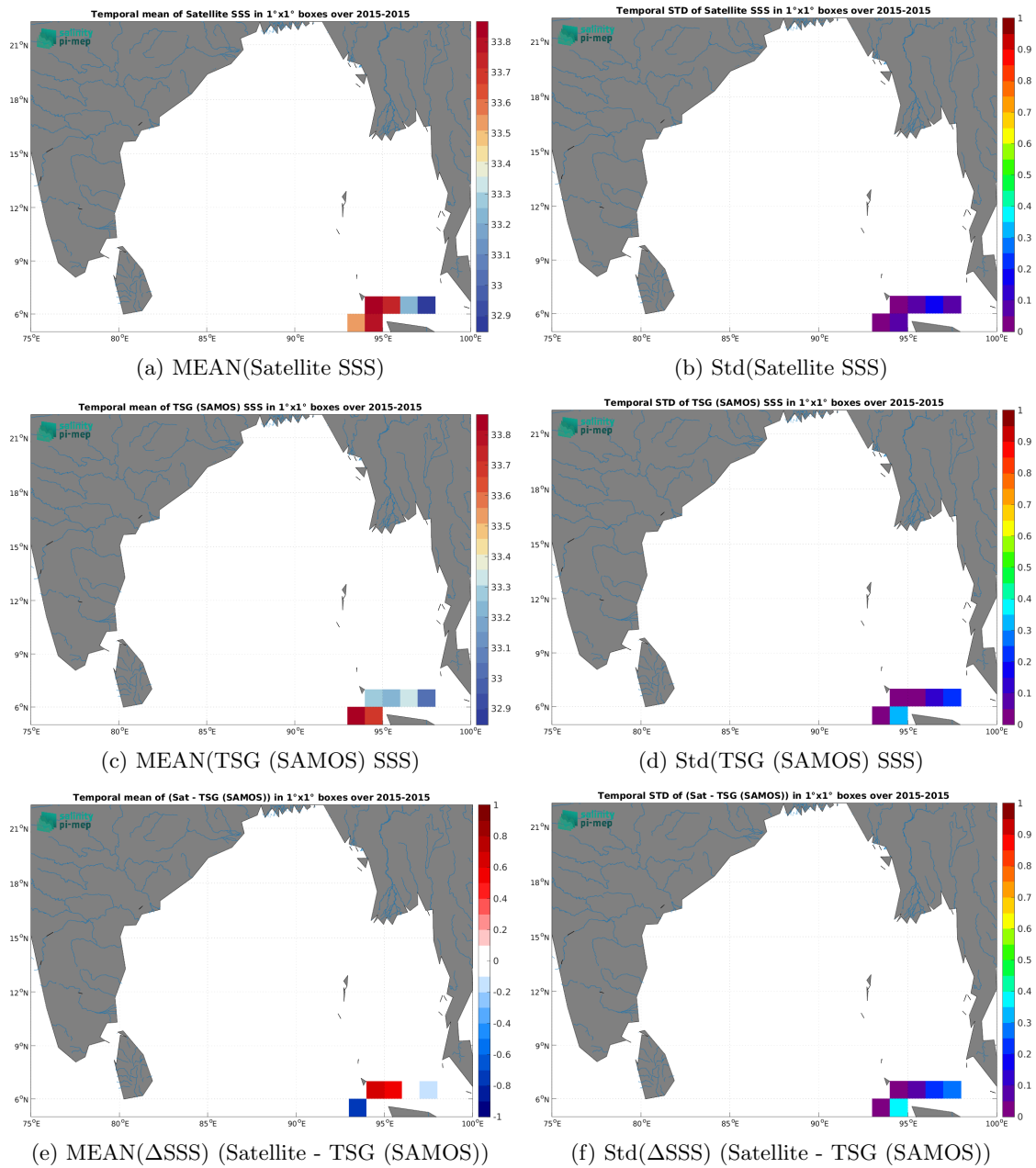
Figure 6: Temporal mean (left) and Std (right) of SSS from SMAP SSS L4 OI v2 - 7 Days (ESR) (top), TSG (SAMOS) (middle), and of \Delta SSS (Satellite - TSG (SAMOS)). Only match-up pairs are used to generate these maps.
